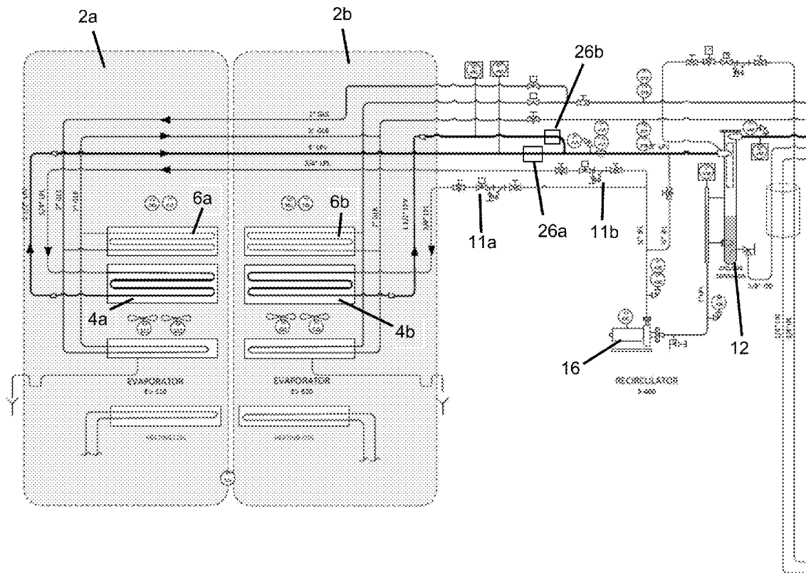
Process and Instrumentation Diagram
