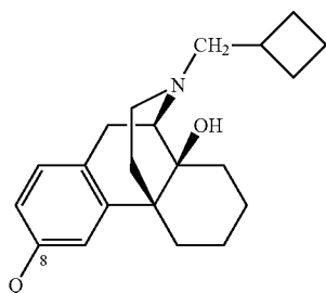
Butorphanol core
