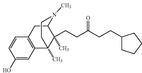
WIN 44, 441
