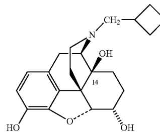
Nalbuphine
