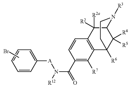
Scheme 3
