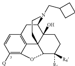
Nalbuphine core
