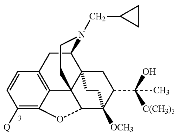
Buprenorphine core
