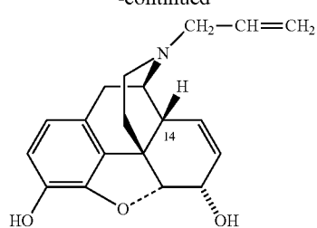
Nalorphine
