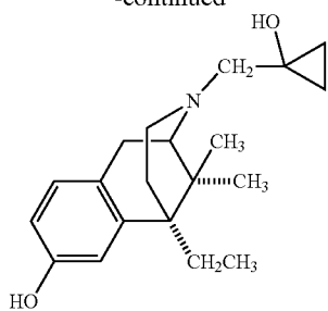
Bremazocine
