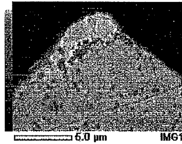
FIG.30A COMPO image
