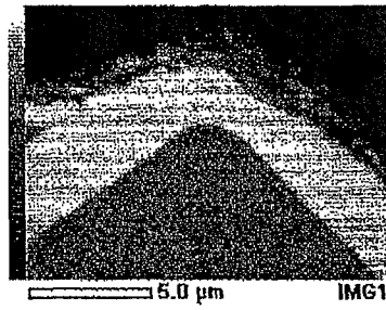
FIG.20A COMPO image
