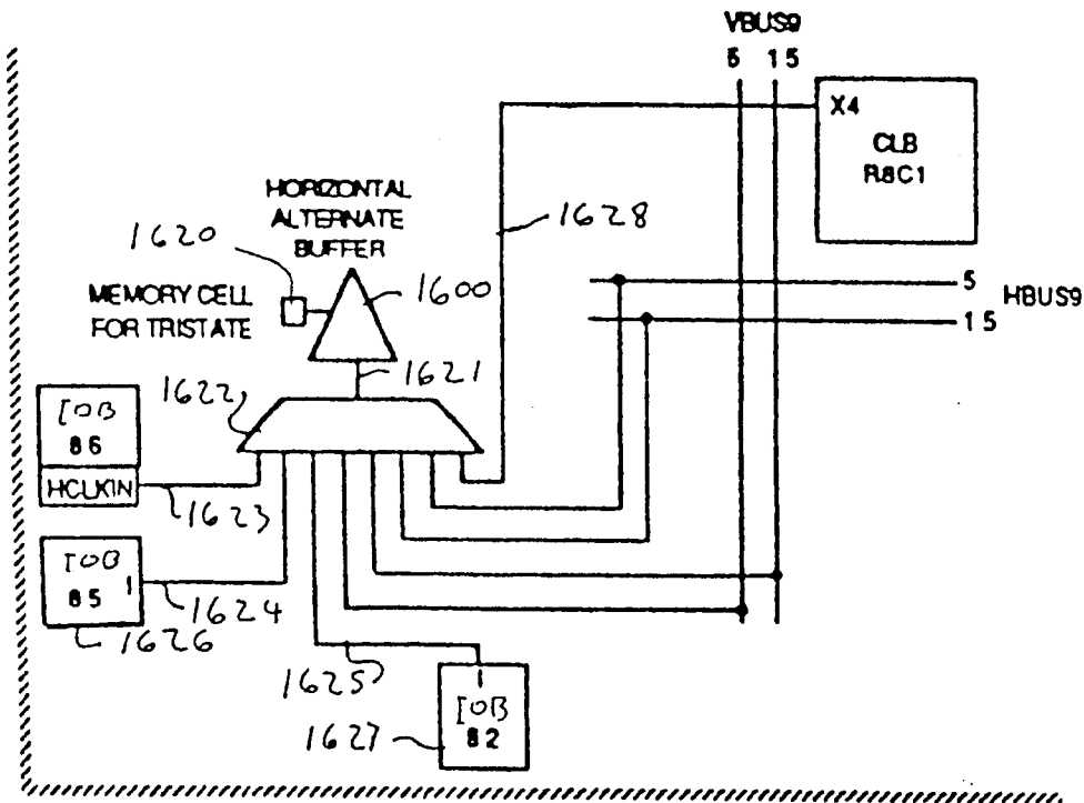
Inputs to the Horizontal Alternate Buffer FIG.-16C
