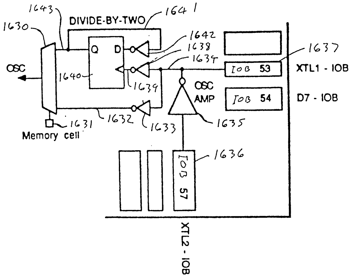
Crystal oscillator
