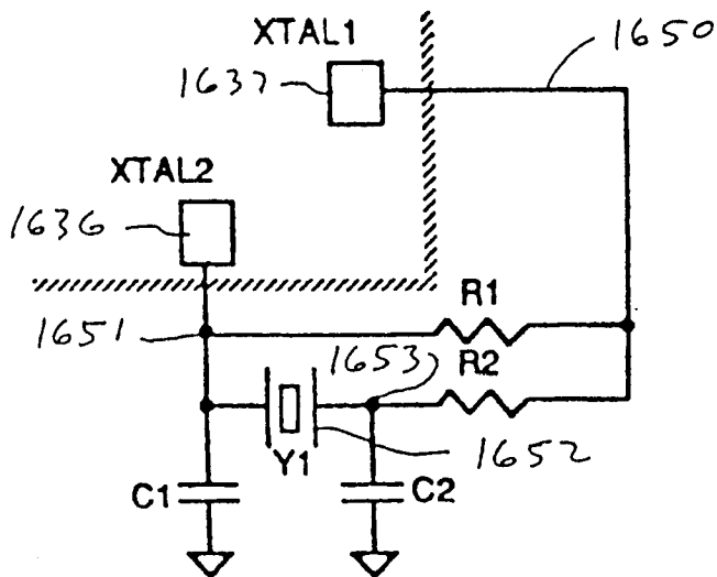
Crystal components
