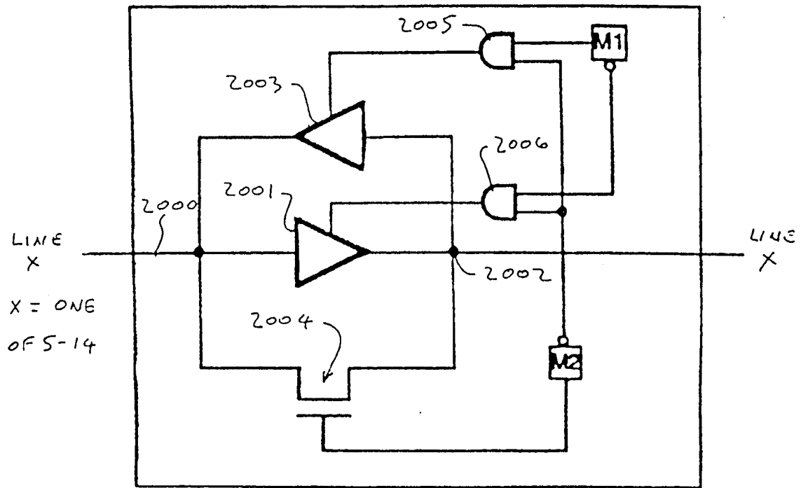
REPOWERING BUFFER
