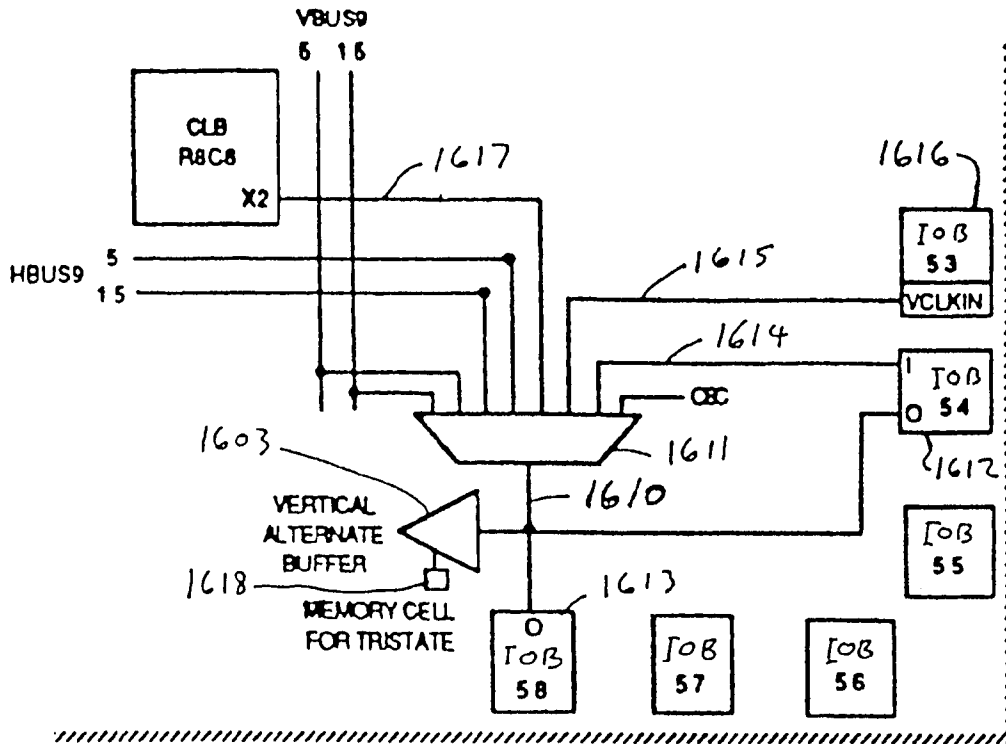
Inputs to the Vertical Alternate Buffer FIG.-16B
