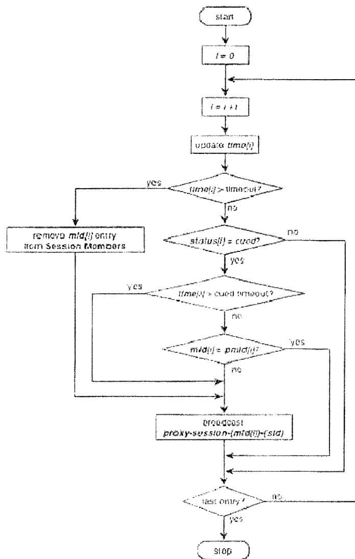
Prune Session Members Flow Diagram
