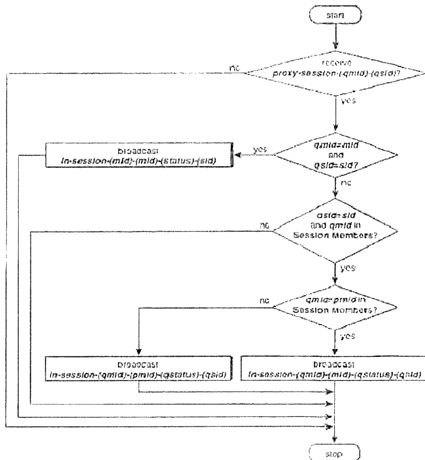
Service Proxy Requests Flow Diagram
