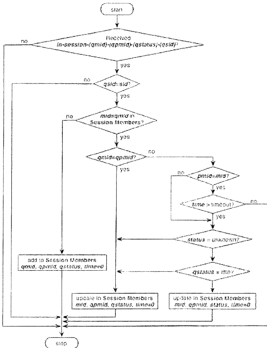
Update Session Members Flow Diagram
