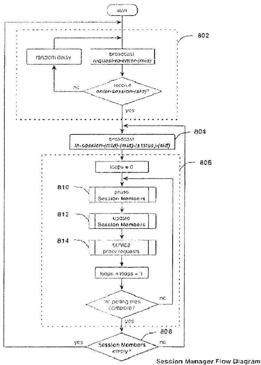
Session Manager Flow Diagram
