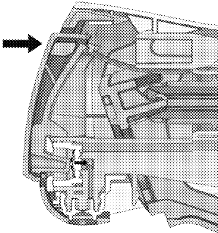
Dome valve closing.
