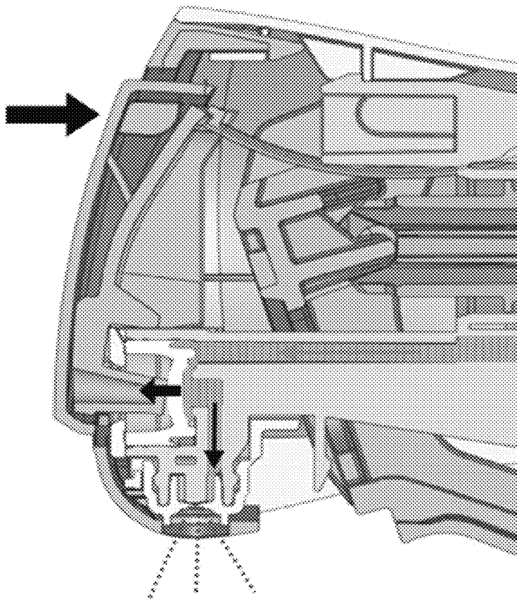
Dome valve opening.
