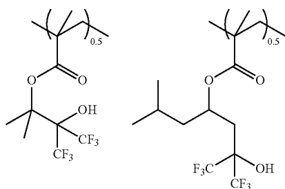
Water-repellent polymer 1
