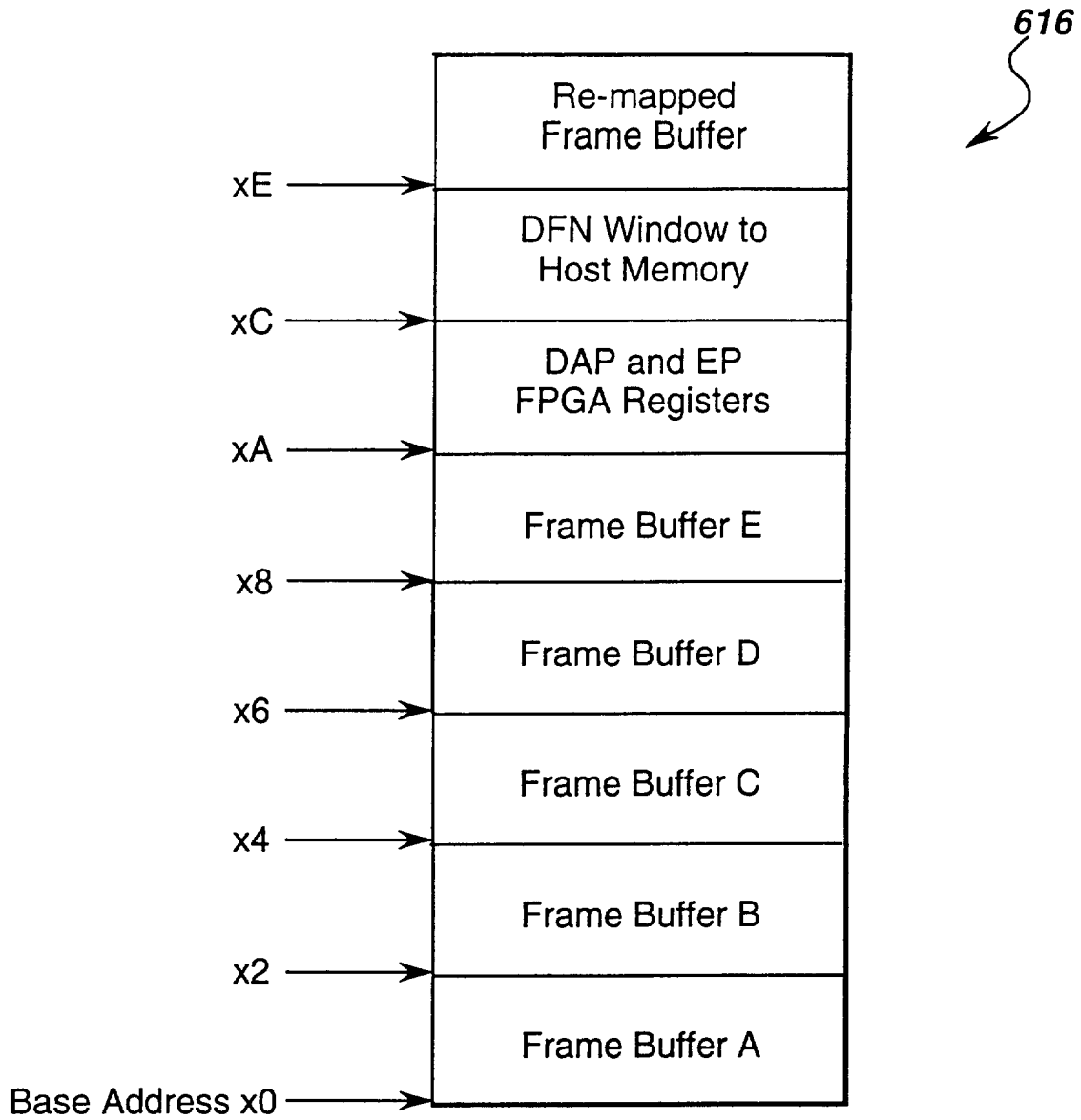
Mapping of 16 MByte PCI Address Space
