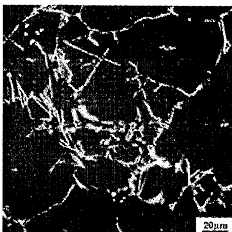
PI1 – MEV secondary electrons
