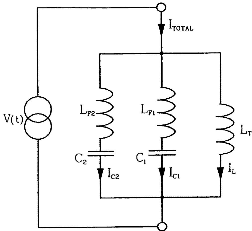
FIGURE 3-4 TANK CIRCUIT WITH TWO RESONANCES
