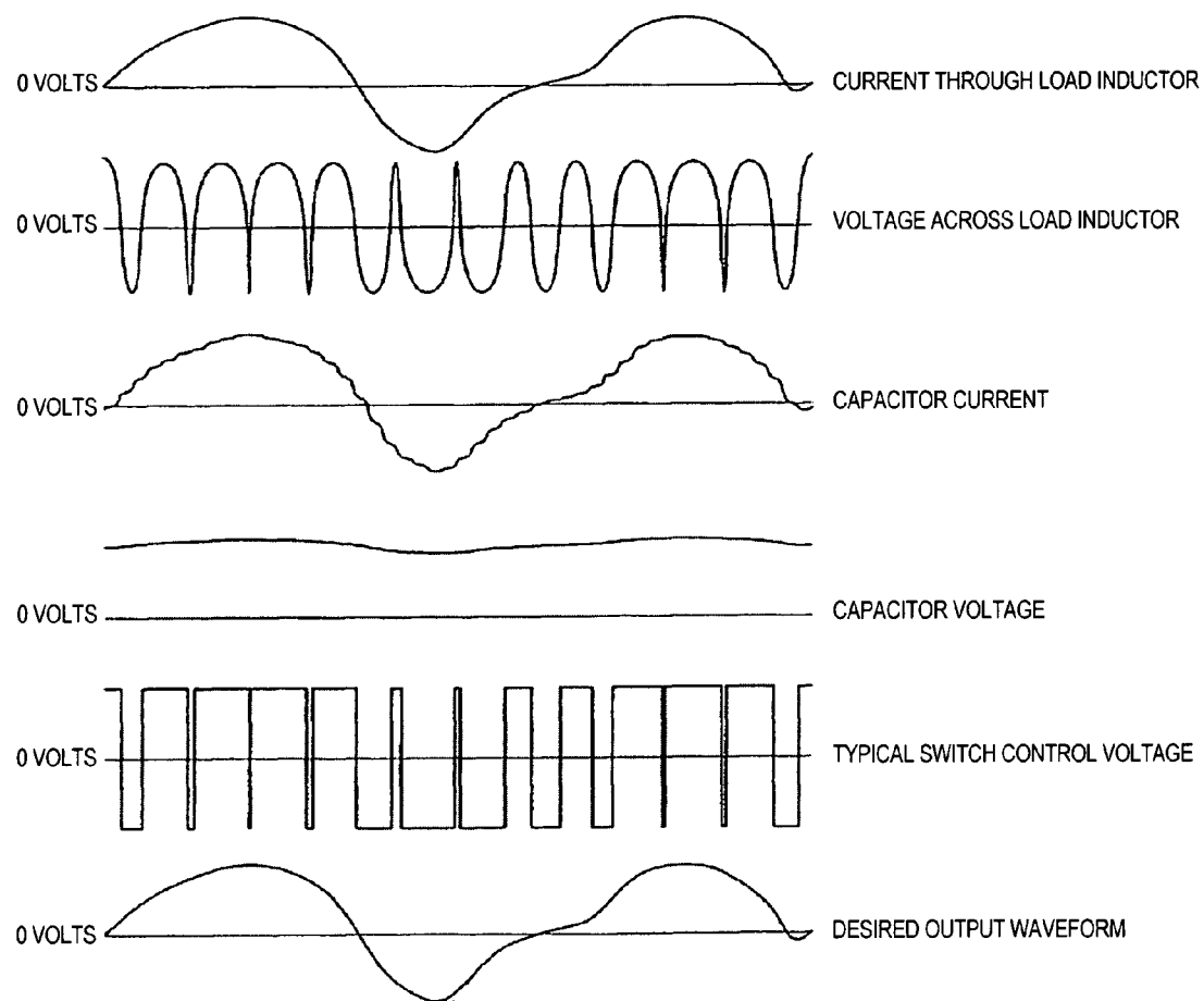
FIGURE 4-3 SWITCHED CAPACITOR CIRCUIT WAVEFORMS
