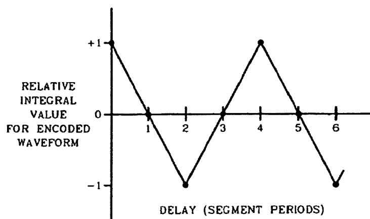
FIGURE 6-2 CORRELATION OF THE 4 SEGMENT (+ - - +) ENCODED WAVEFORM WITH ITSELF
