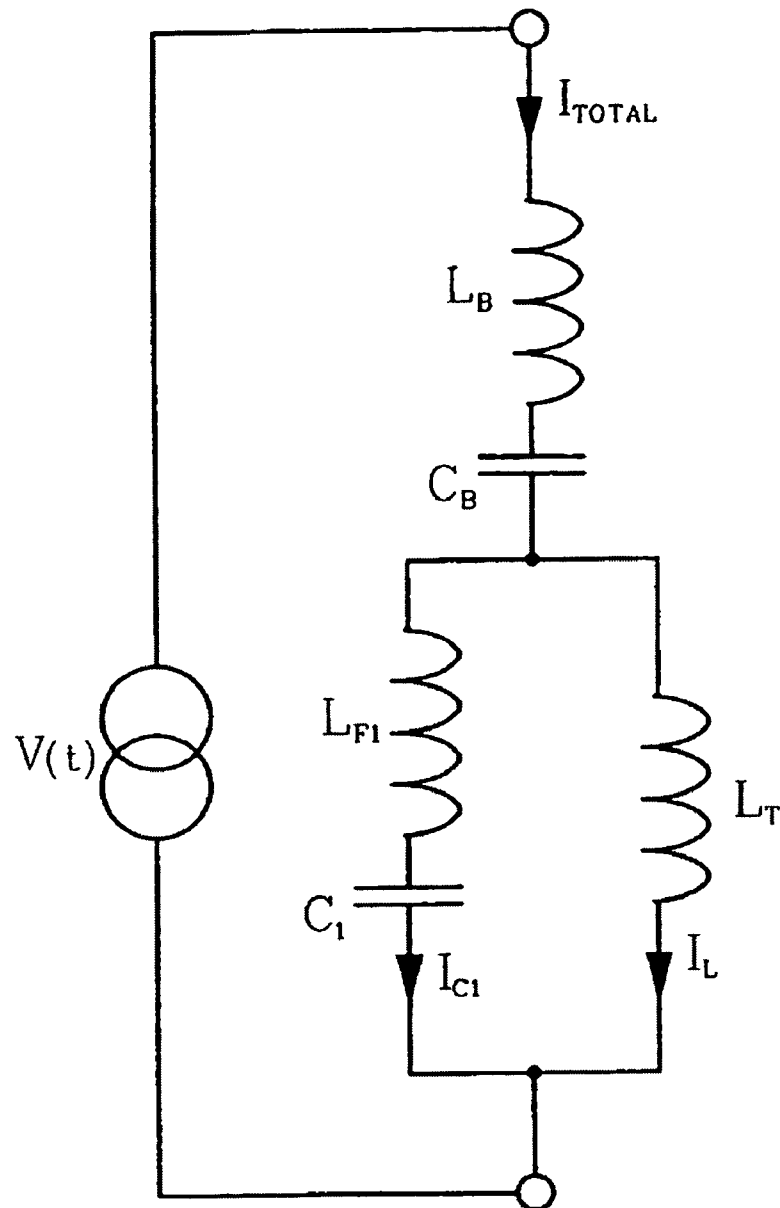
FIGURE 3-5 TANK CIRCUIT WITH SINGLE FREQUENCY BLOCKING CIRCUIT
