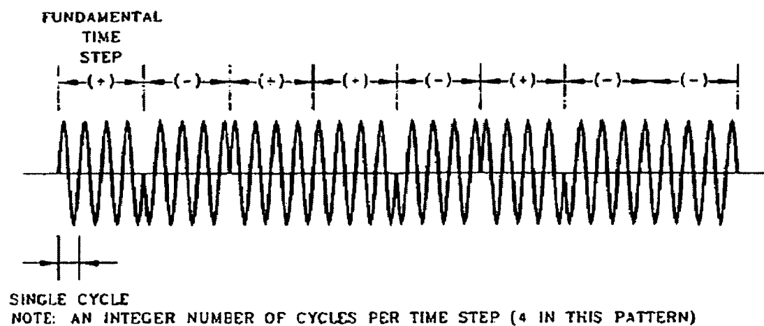
FIGURE 1-10 AN 8 SECTION (+ - + + - + - -) TIME ENCODED WAVEFORM
