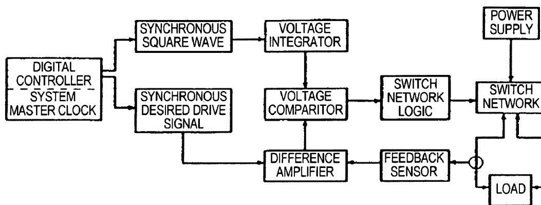
FIGURE 2-1 SYNCHRONOUS PULSE WIDTH MODULATION AMPLIFIER
