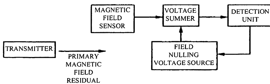
FIGURE 1-4B VOLTAGE NULLING OF RESIDUAL FIELD SENSOR OUTPUT
