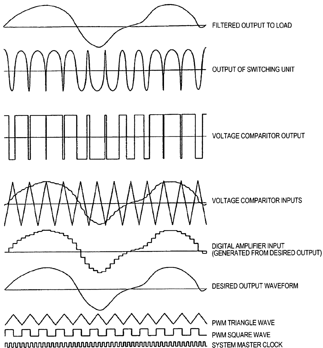
FIGURE 2-2 TYPICAL PULSE WIDTH MODULATION WAVEFORMS
