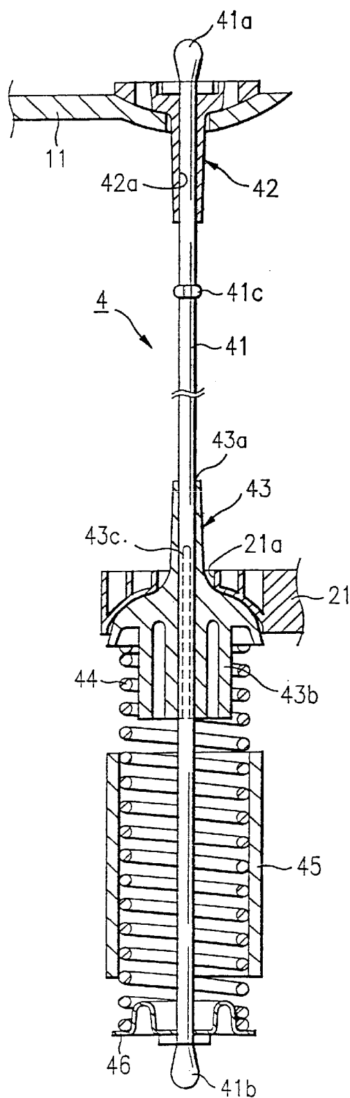
FIG. 2 Prior Art
