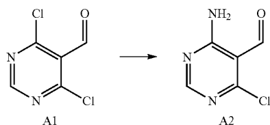
Scheme A
