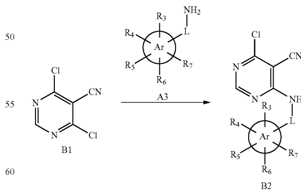
Scheme B
