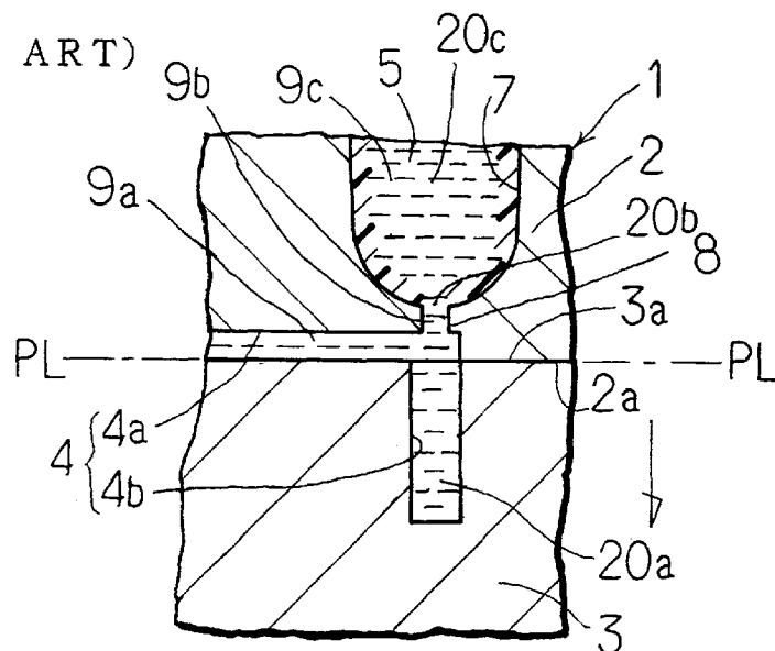
Fig. 13 (PRIOR ART)
