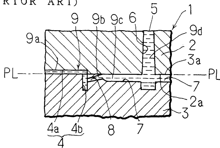
Fig. 12 (PRIOR ART)
