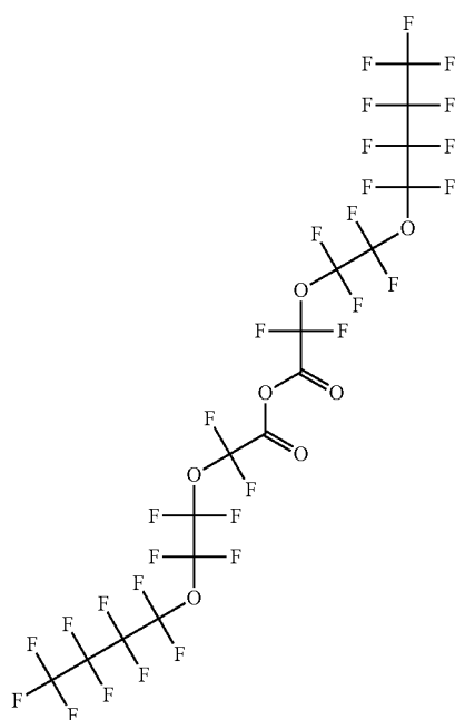
Perfluoro-3,6-dioxadecanoic anhydride
