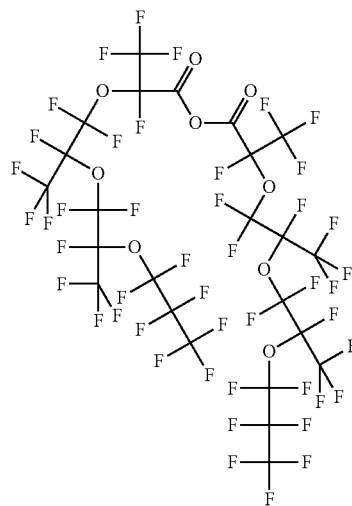
Perfluoro(2,5,8-trimethyl-3,6,9-trioxadodecanoic anhydride)
