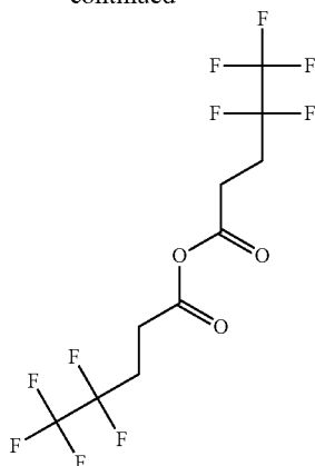
4,4,5,5,5-Pentafluoropentanoic anhydride
