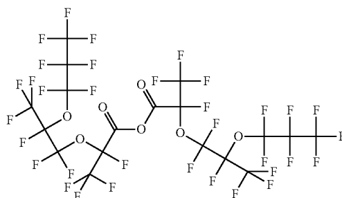
Perfluoro(2,5-dimethyl-3,6-dioxananoic anhydride)
