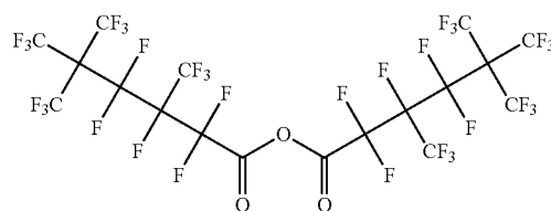
Perfluoro-3,5,5-trimethylhexanoic anhydride
