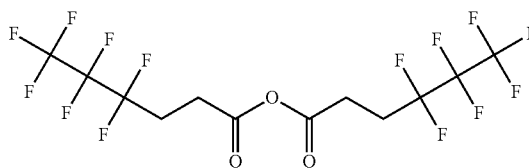
4,4,5,5,6,6,6-Heptafluorohexanoic anhydride
