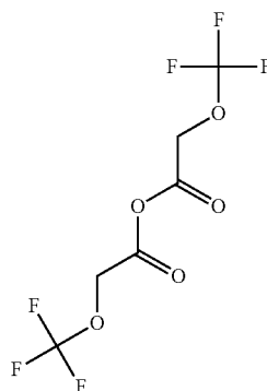
2-(Trifluoromethoxy)acetic anhydride
