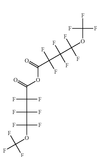
Perfluoro(4-methoxybutanoic) anhydride
