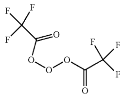
Trifluoroperacetic anhydride
