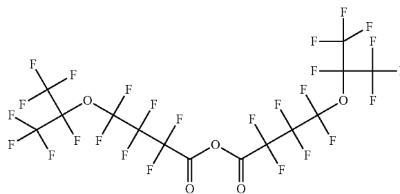
4-(Heptafluoroisopropoxy)hexafluorobutanoic anhydride
