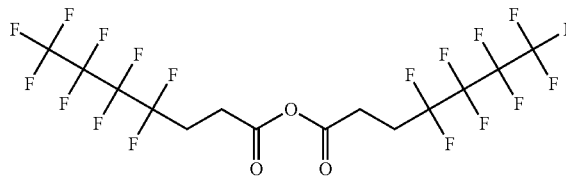
4,4,5,5,6,6,7,7,7-Nonafluoroheptanoic anhydride
