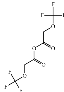
2-(Trifluoromethoxy)acetic anhydride
