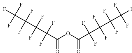
Nonafluoropentanoic anhydride
