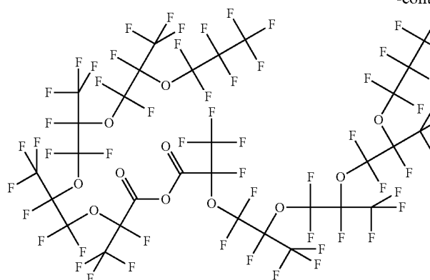
Perfluoro(2,5,8,11-tetramethyl-3,6,9,12-tetraoxopentadecanoic) anhydride
