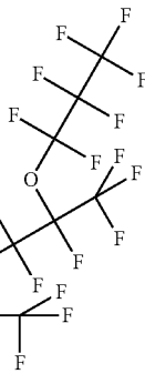
Perfluoro(2,5,8,11-tetramethyl-3,6,9,12-tetraoxopentadecanoic) anhydride
