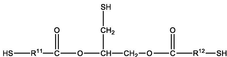
Formula (K)
