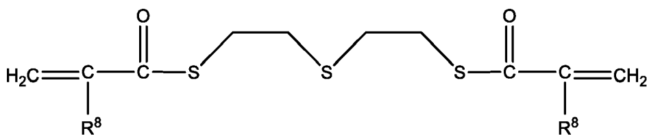
Formula (IIb)
