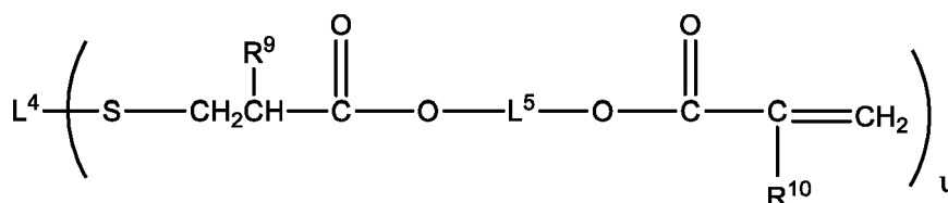
Formula (III)
