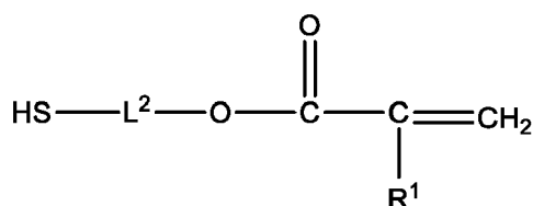
Formula (F)
