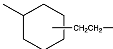
Formula (G-2)
