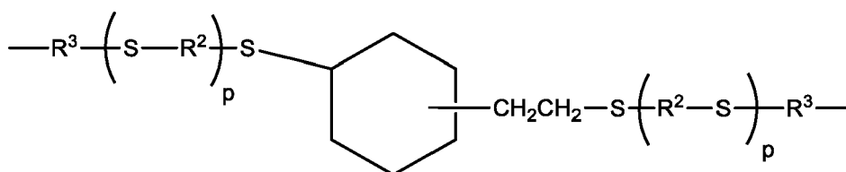
Formula (G-3)
