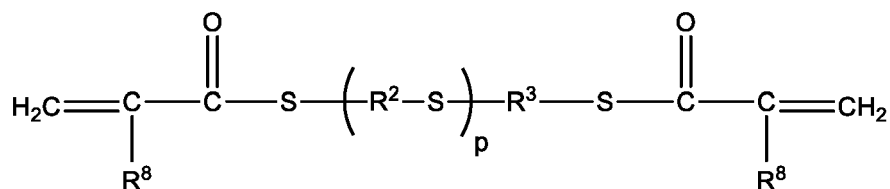
Formula (IIa)
