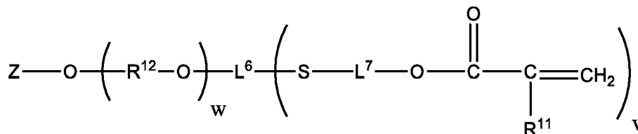
Formula (IV)
