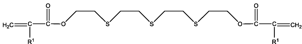
Formula (Ib)
