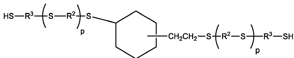
Formula (N-2)
