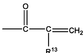
Formula (V)
