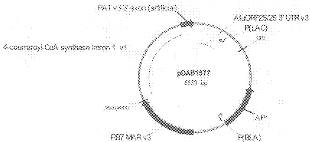
Figure 17: Schematic representation of plasmid pDAB1577
