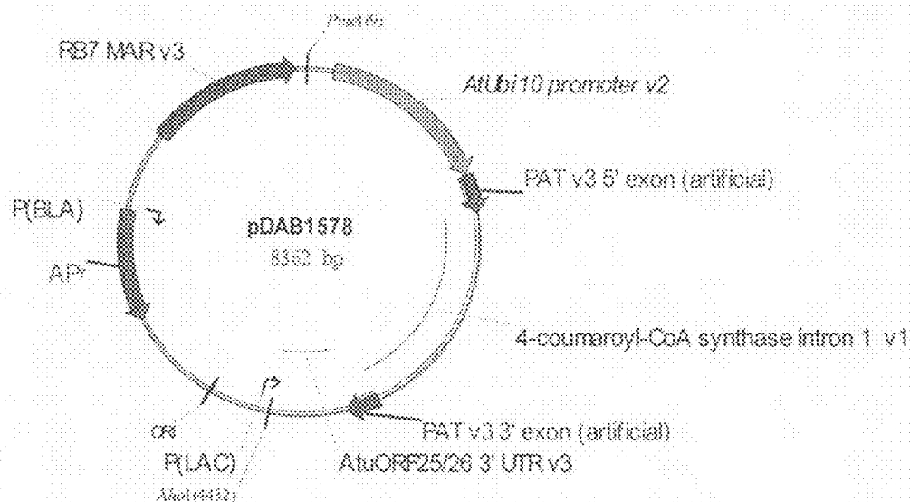
Figure 57: Schematic representation of plasmid pDAB1578
