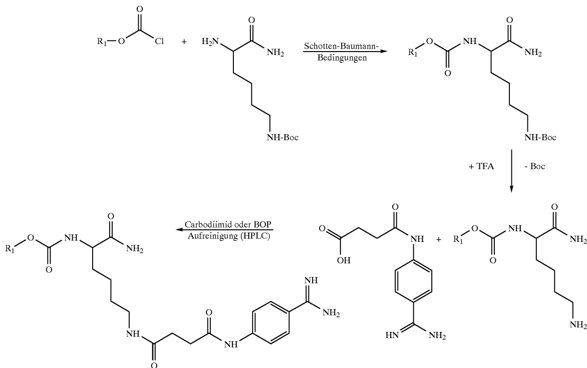
Scheme 5: Reaction with chloroformic acid esters
