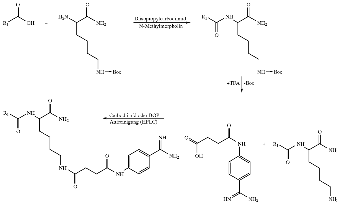
Scheme 4: Reaction with carboxylic acids
