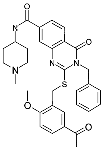
Compound 2012
