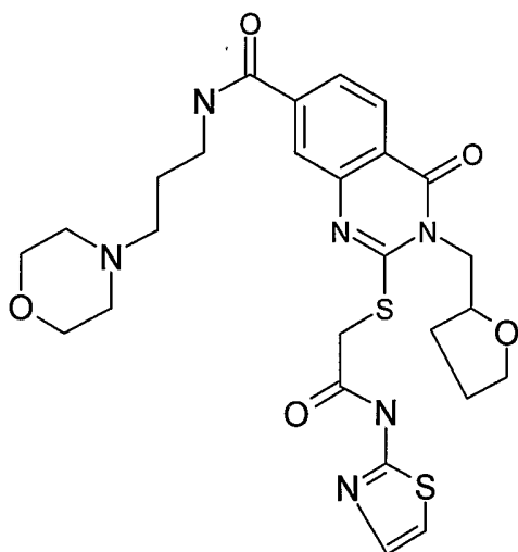
Compound 6
