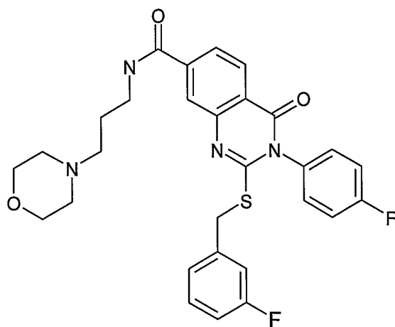
Compound 3
