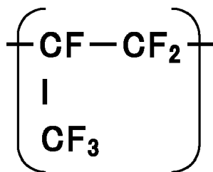
HFP (hexafluoropropylene)
