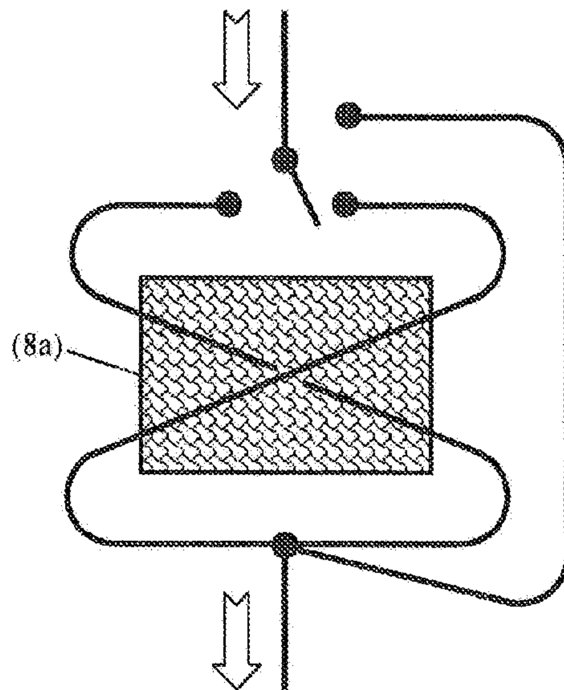
Figure 2 ... Paths through/around heat exchanger.
