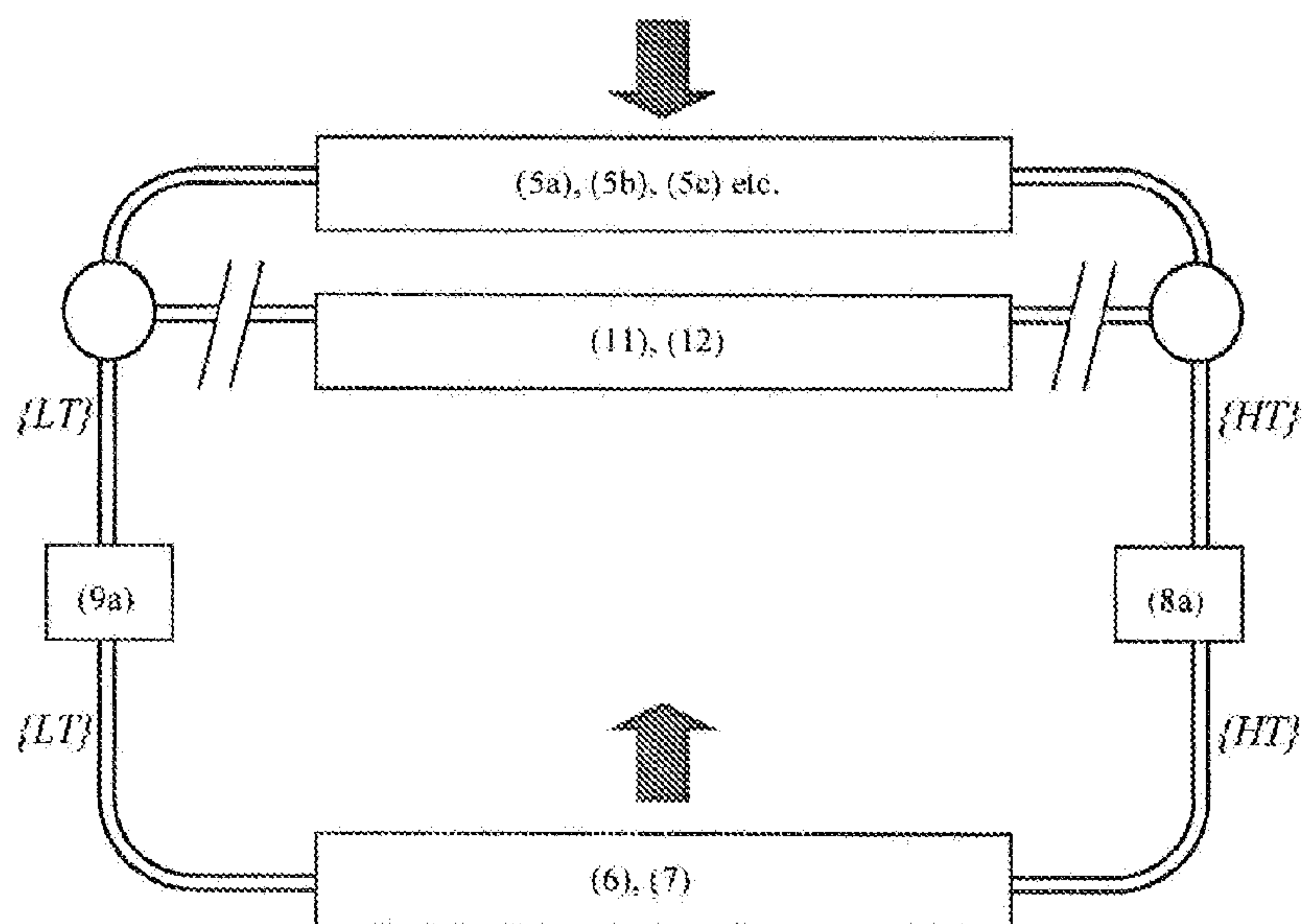
Figure 3 ... Exergy Flows in Operating Mode (a).
