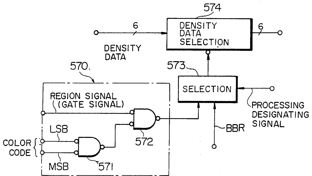
500B: DATA SELECTING CIRCUIT
