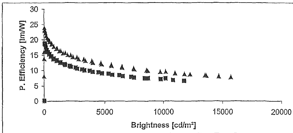
Figure 2: Power efficiency as a function of brightness
