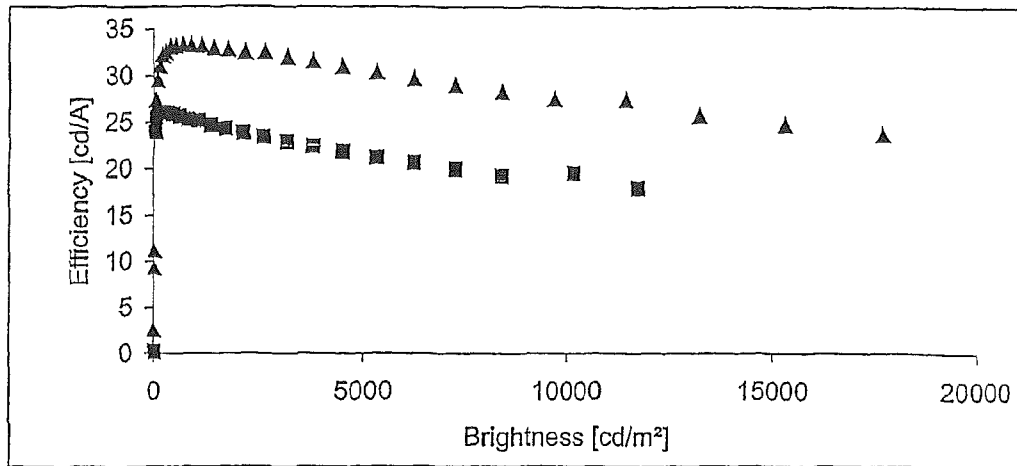
Figure 1: Efficiency as a function of brightness
