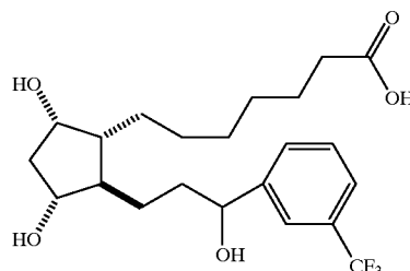
13,14-dihydro-15-(3-trifluoromethylphenyl)-15-pentanor Prostaglandin \text{F}_1\alpha
