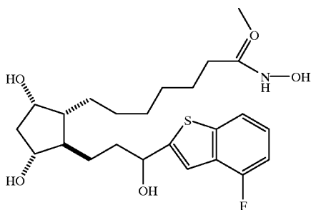
13,14-dihydro-15-(5-fluorothianaphthyl)-15-pentanoic acid Prostaglandin F 1 α 1-hydroxamic acid
