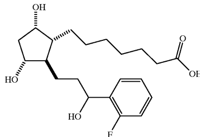
13,14-dihydro-15-(2-fluorophenyl)-15-pentanor Prostaglandin \text{F}_1\alpha
