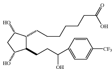
13,14-dihydro-15-(4-trifluoromethylphenyl)-15-pentanor Prostaglandin \text{F}_1\alpha
