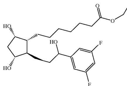
13,14-dihydro-15-(3,5 difluorophenyl)-15-pentanor Prostaglandin \text{F}_1\alpha ethyl ester
