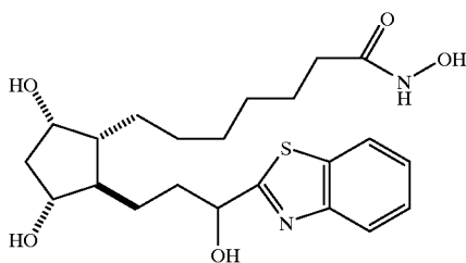
13,14-dihydro-15-(benzothiazolyl)-15-pentanoic acid Prostaglandin F 1 α 1-hydroxamic acid
