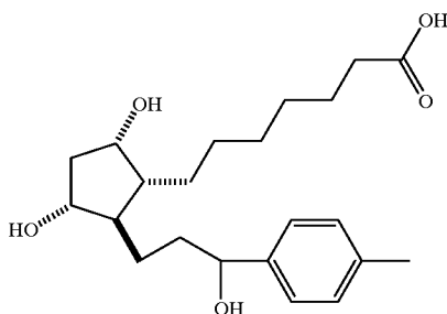
13,14-dihydro-15-(4-methylphenyl)-15-pentanor Prostaglandin \text{F}_1\alpha
