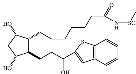
13,14-dihydro-15thianaphthyl-15-pentanoic acid Prostaglandin F 1 α 1-N-methanesulfonamide
