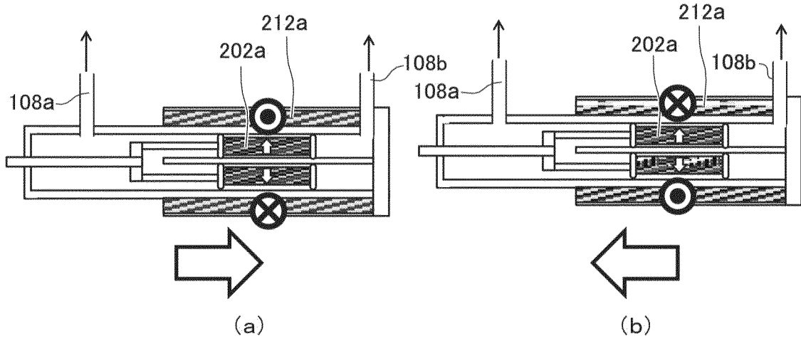
SINGLE PHASE DRIVE
