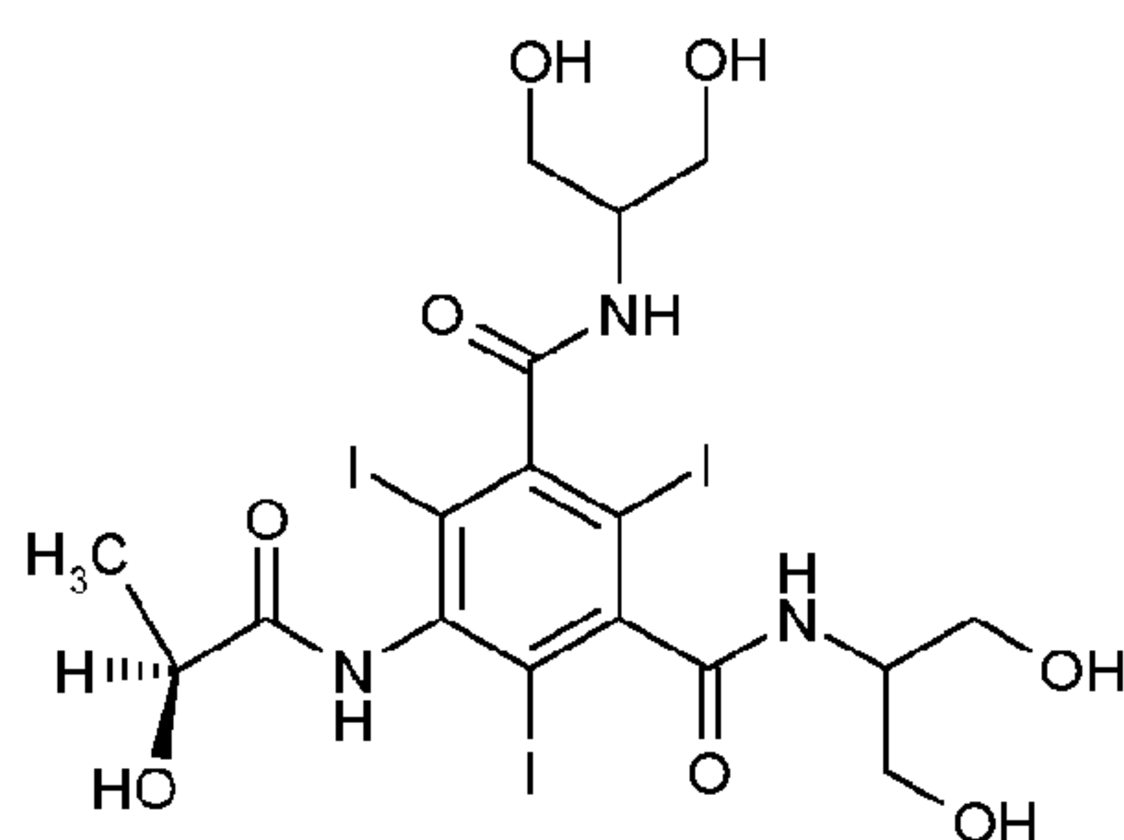
Iopamidol
