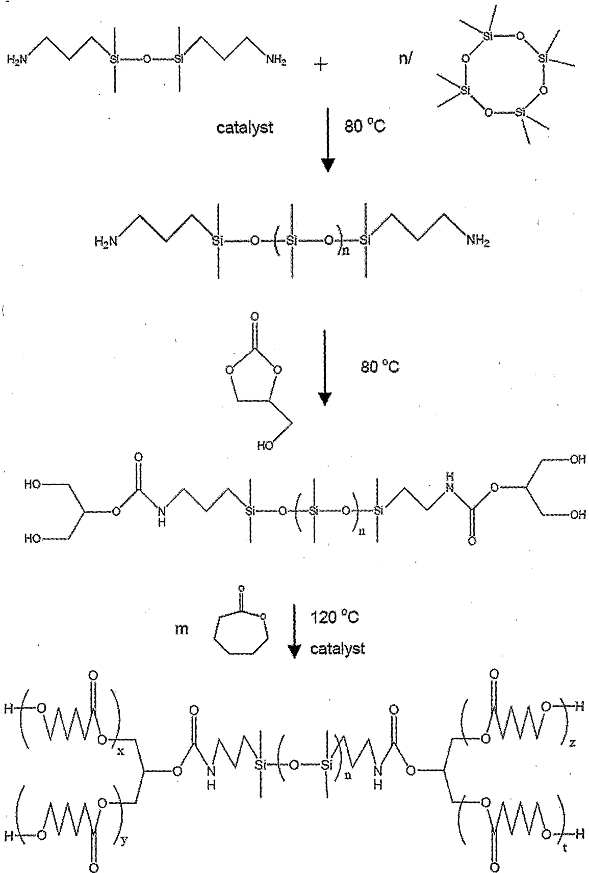
Scheme 1: Synthesis scheme of carbamate linked tetra functional PDMS oligomers and block copolymers.
