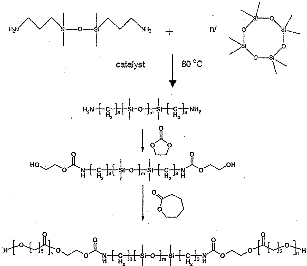
Scheme 2: Synthesis scheme of carbamate linked di functional PDMS oligomers and block copolymers.
