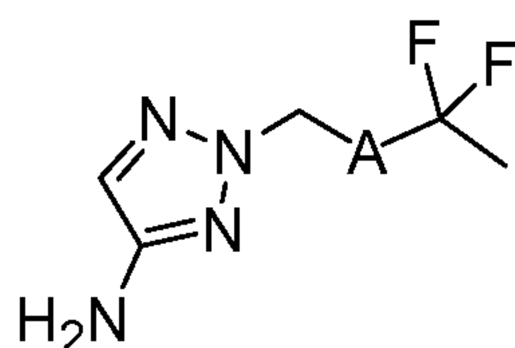
Structure 1
