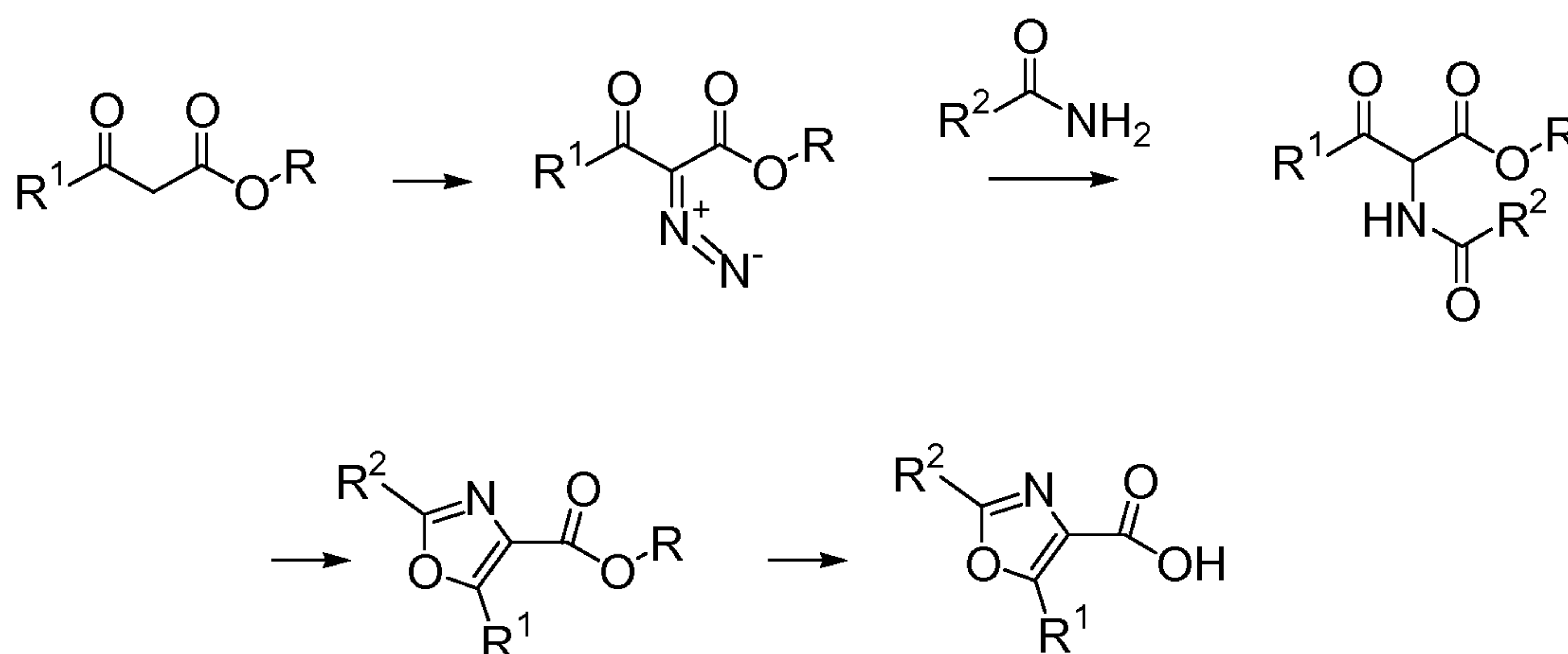
Scheme 2: Oxazole synthesis (2).
