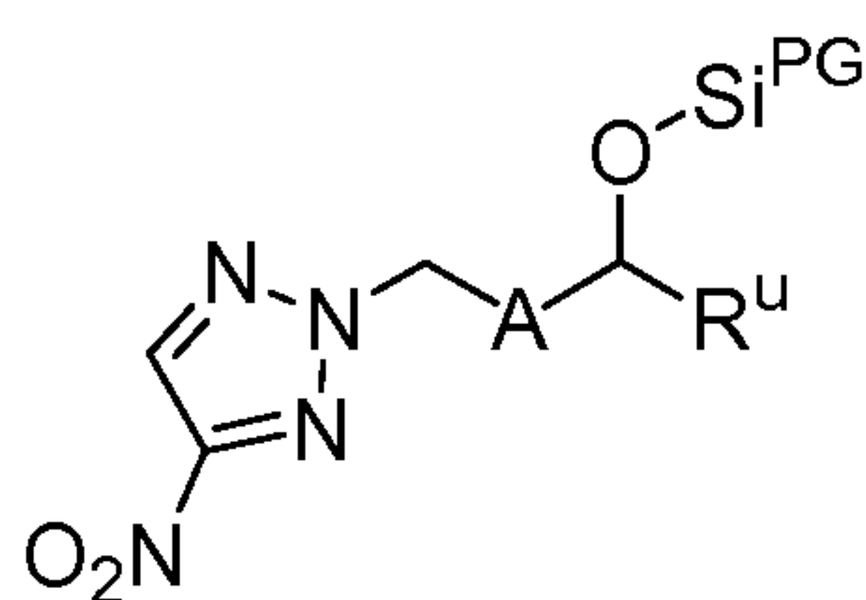
Structure 6
