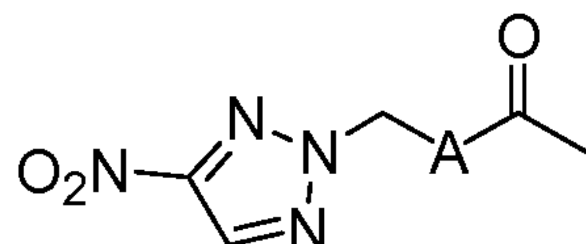
Structure 3
