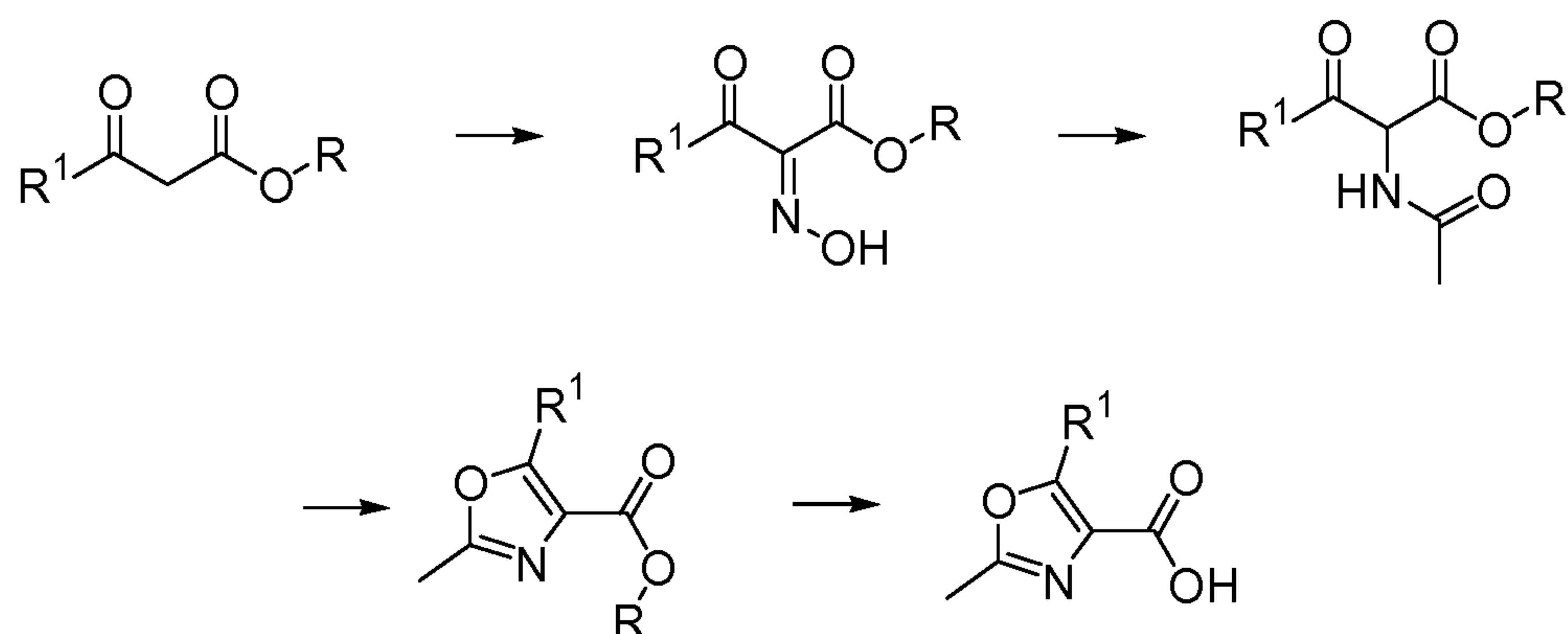
Scheme 1: Oxazole synthesis (1).
