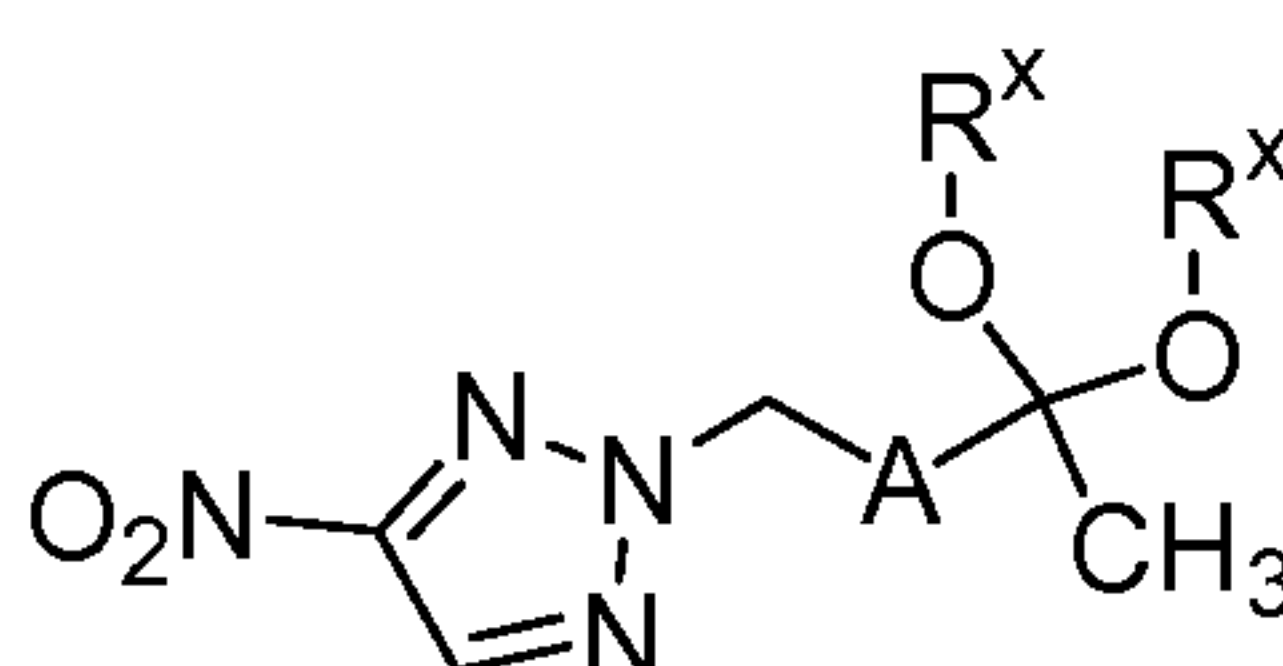
Structure 4
