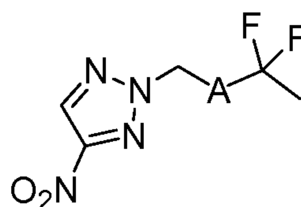
Structure 2
