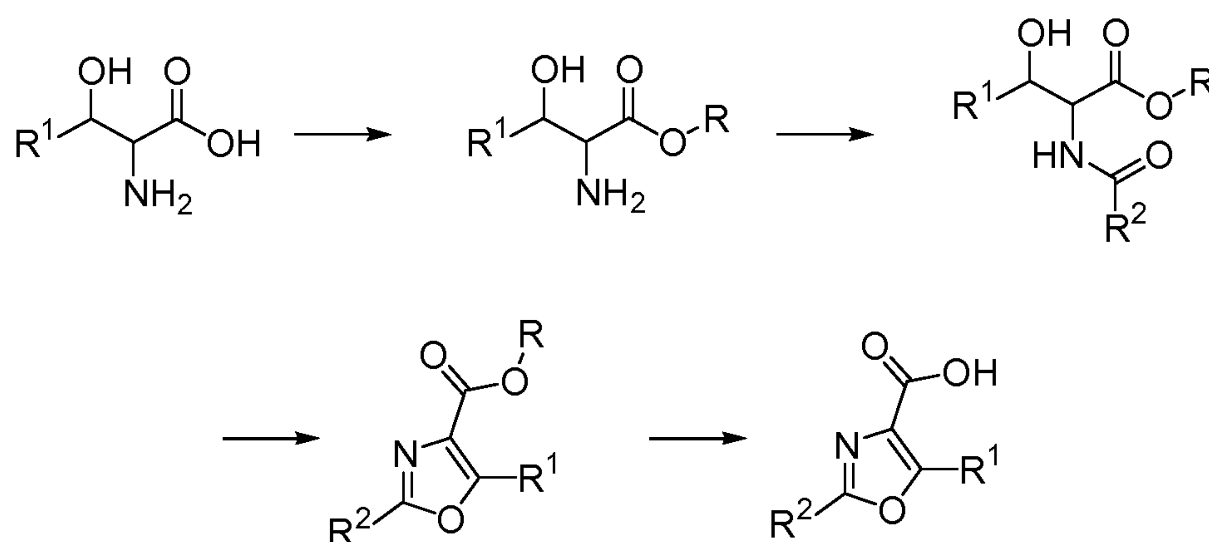
Scheme 3: Oxazole synthesis (4).
