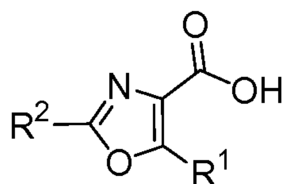
Structure 7
