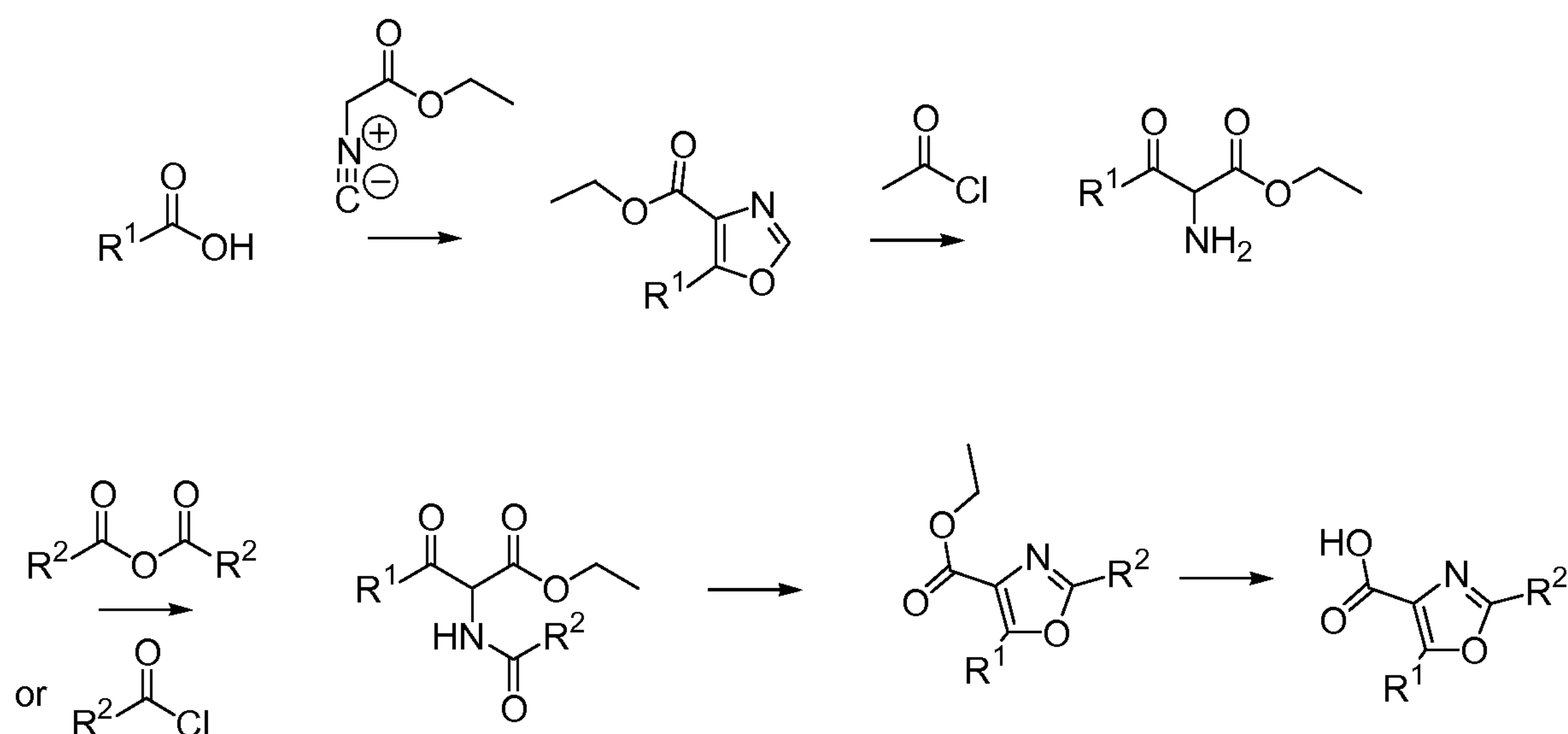
Scheme 4: Oxazole synthesis (5).
