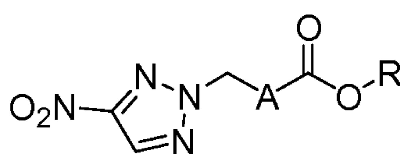
Structure 5
