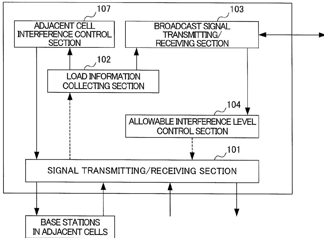
BASE STATION BS1 IN RADIO COMMUNICATION SYSTEM 1
