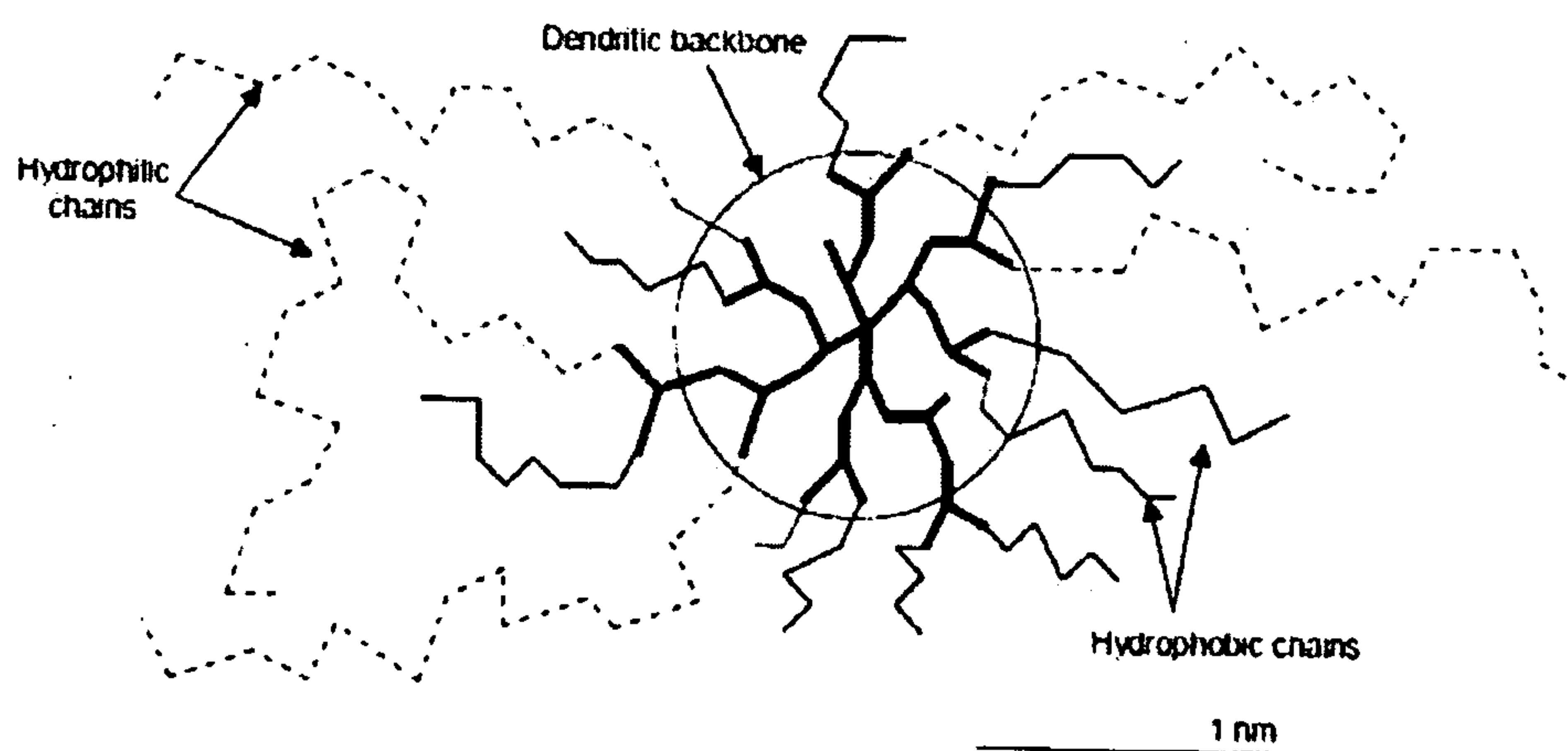
Hyperbranched polyester with amphiphilic terminal groups.
