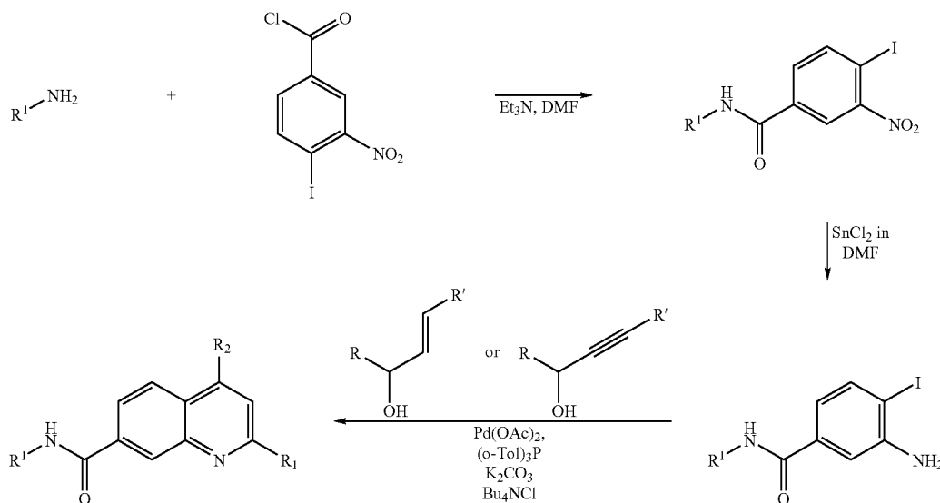
Synthetic scheme 2:
