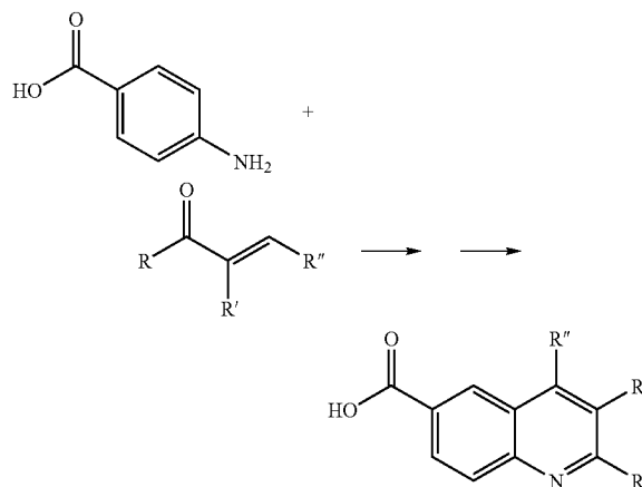
Synthetic scheme 1:
