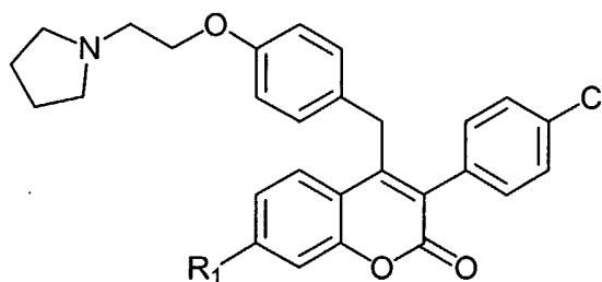
7-substituted 3-(4-chlorophenyl)-4-[4-(2-pyrrolidin-1-yl-ethoxy)-benzyl]-chromen-2-one analogs
