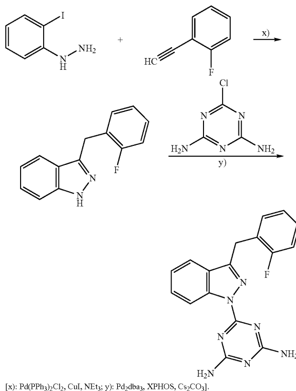
Scheme 7
