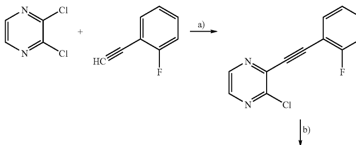
Scheme 1
