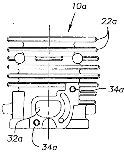
FIG. 8 PRIOR ART
