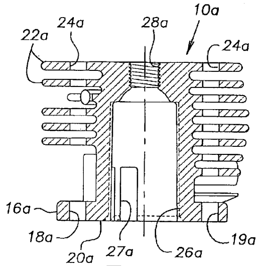
FIG. 7 PRIOR ART
