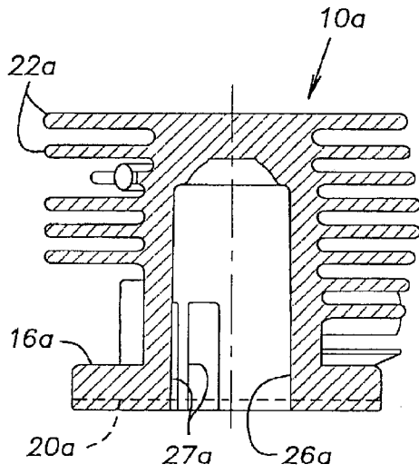
FIG. 6 PRIOR ART
