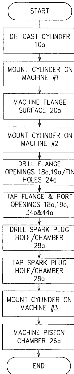
FIG. 10 PRIOR ART
