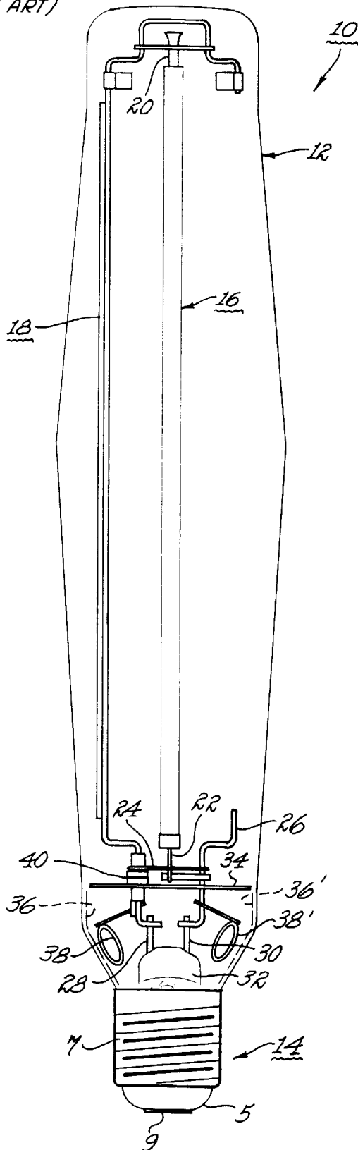
Fig. 1 (PRIOR ART)
