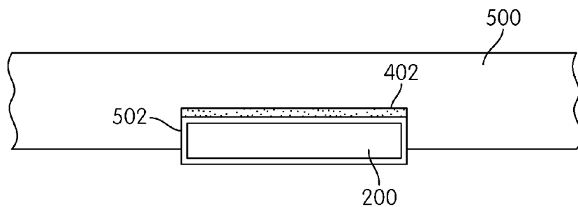
FIG. 5 PRIOR ART
