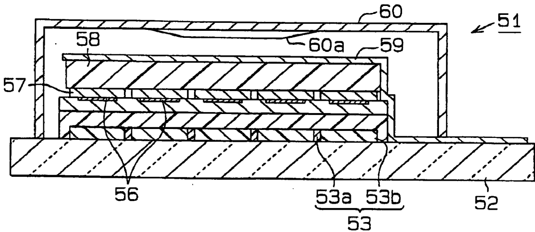
Fig. 4 (Prior Art)
