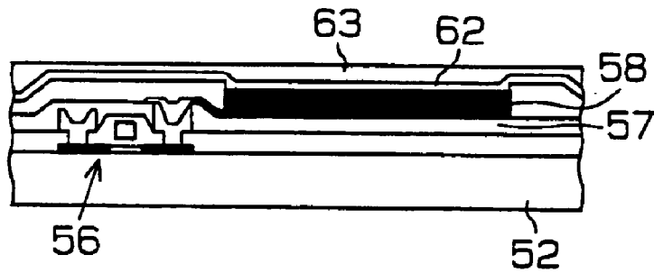
Fig.5 (Prior Art)
