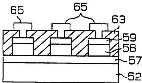
Fig.7 (Prior Art)
