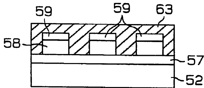
Fig.6 (Prior Art)
