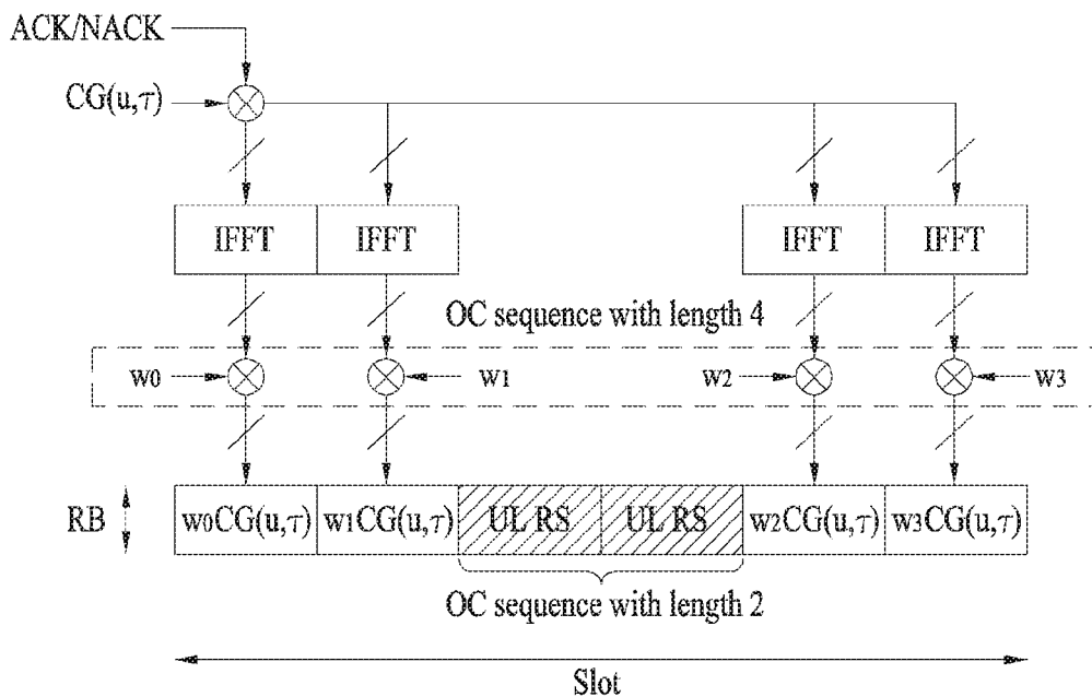
PUCCH format 1a/1b structure (extended CP)
