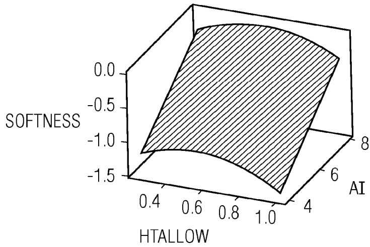
SURFACE PLOT OF SOFTNESS VS AI, HTALLOW
