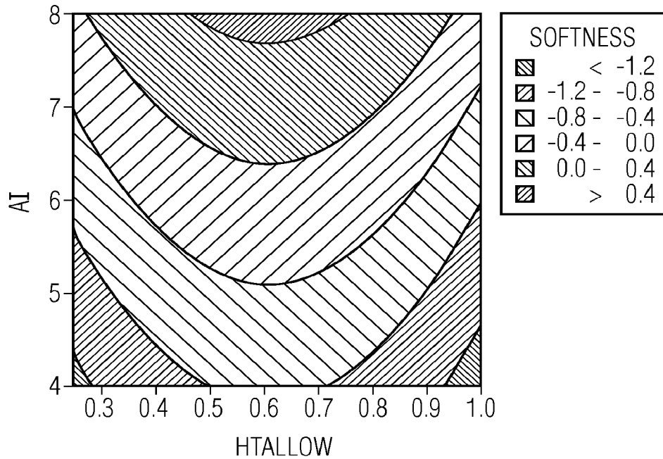
CONTOUR PLOT OF SOFTNESS VS AI, HTALLOW
