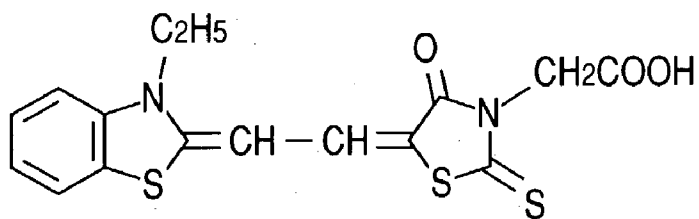
MEROCYANINE
