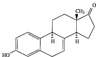
EQUILIN (III) ( \Delta^7 -Dehydroestrone)
