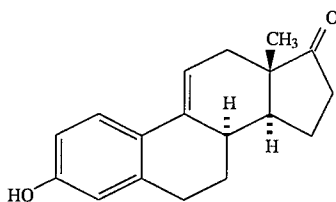
A9(11)-Dehydro-8-isoestrone (VI)
