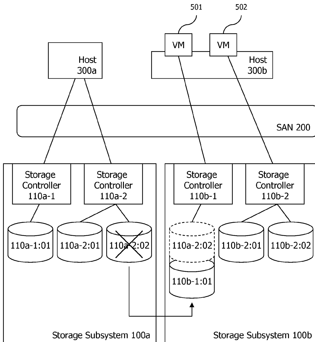
Fig.9 System Configuration (logical view)
