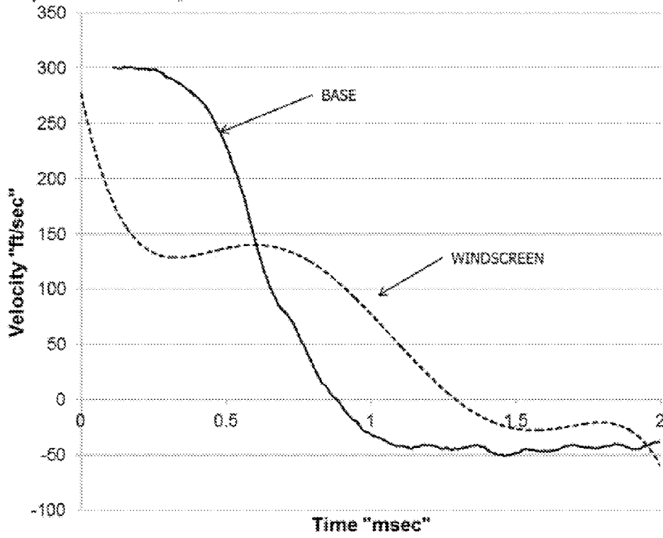
Velocity Curves, @300ft/sec
