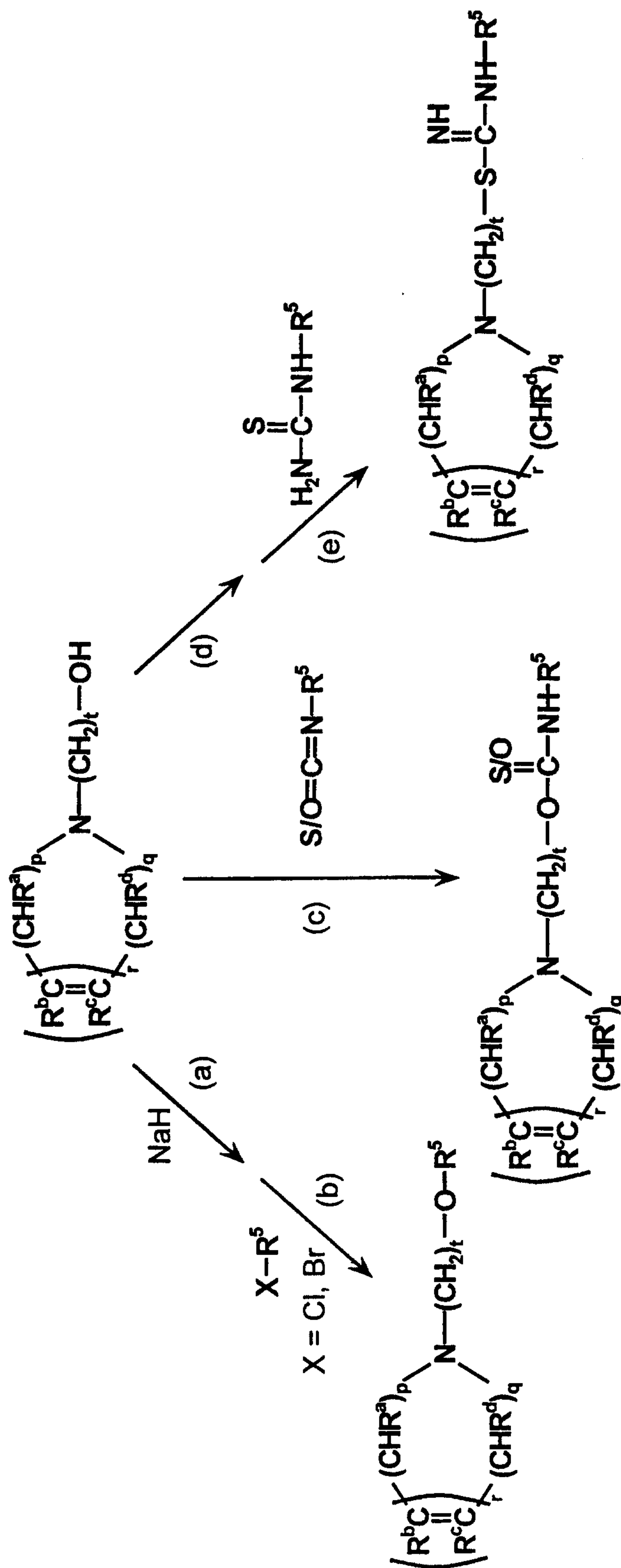
SCHEME 8:
