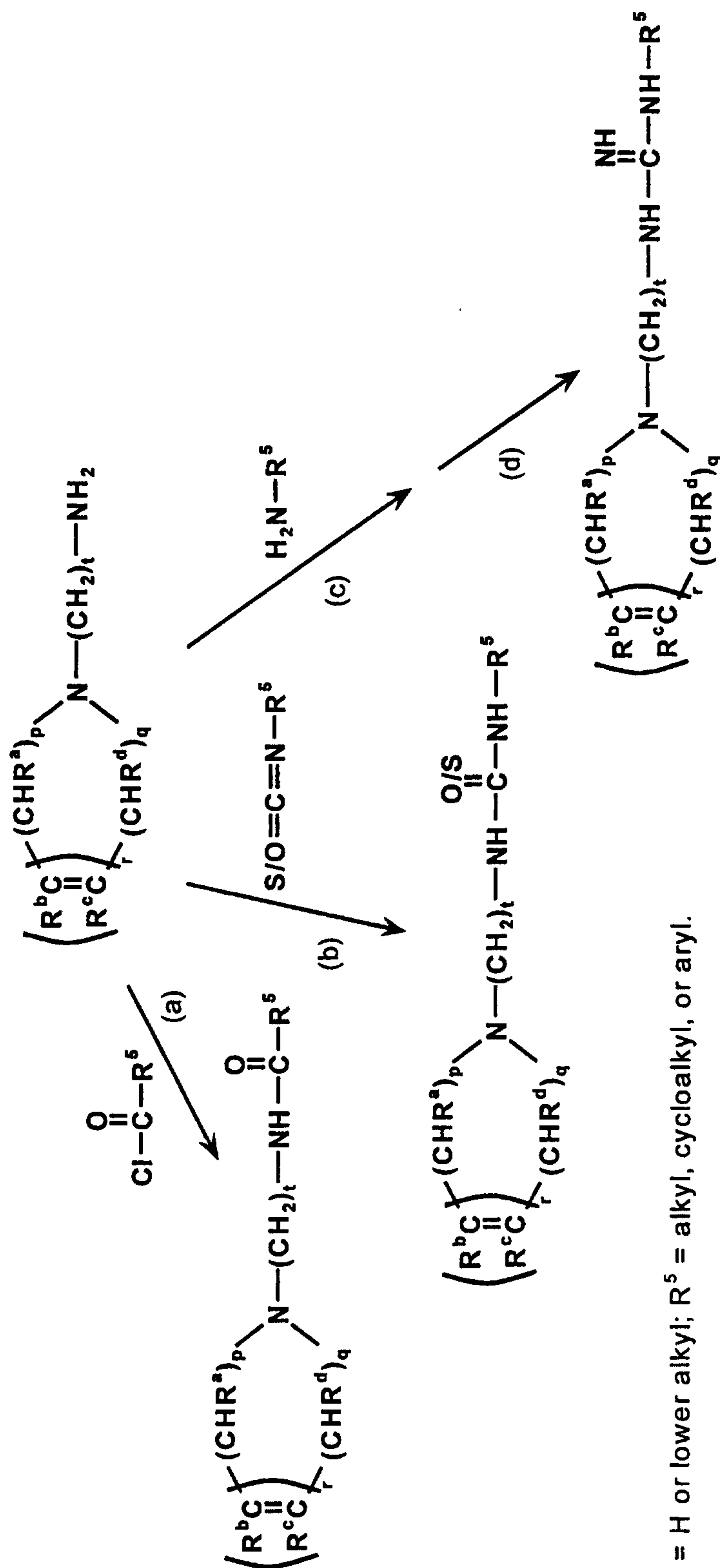
SCHEME 7:
