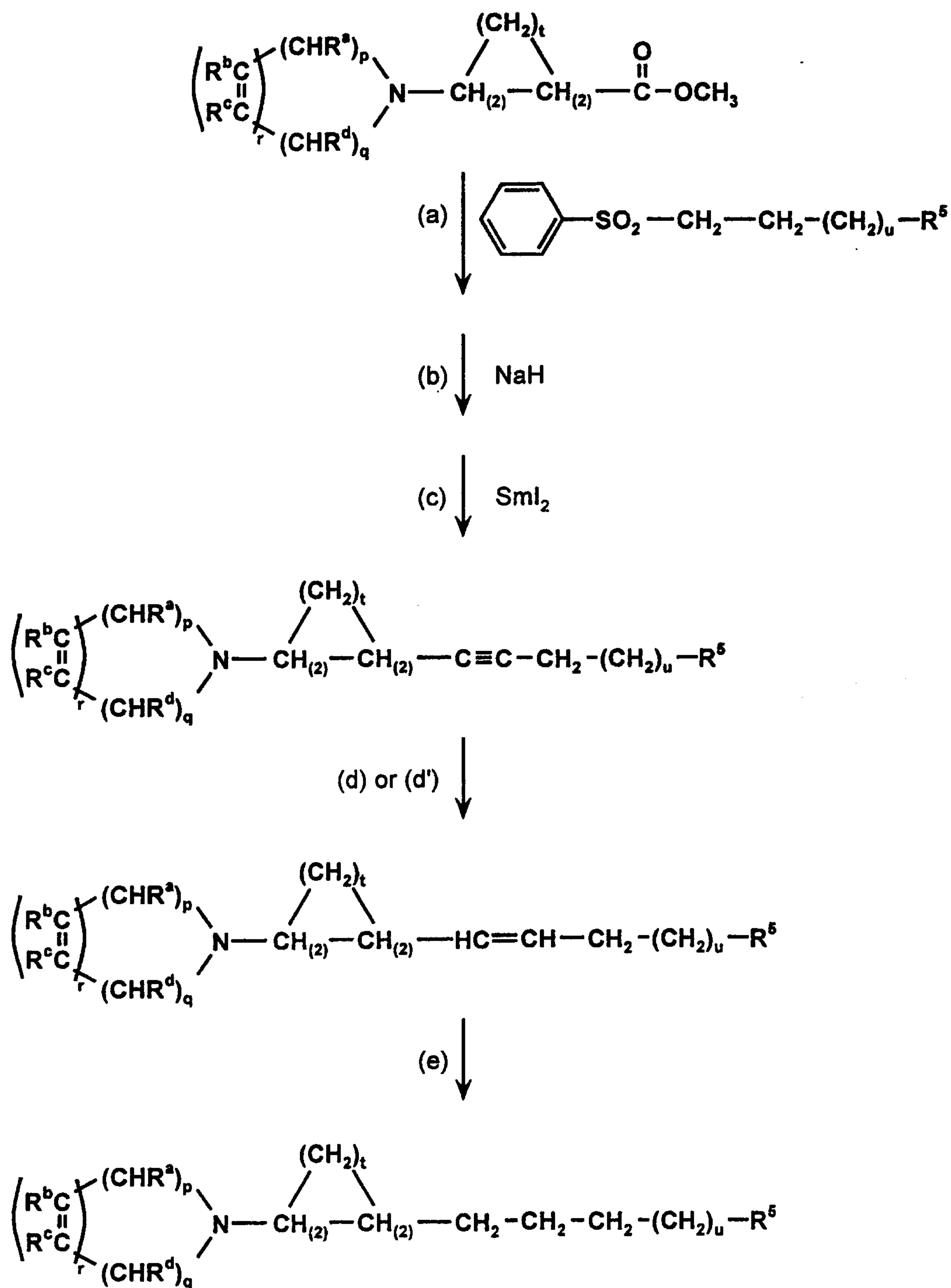
SCHEME 14:
