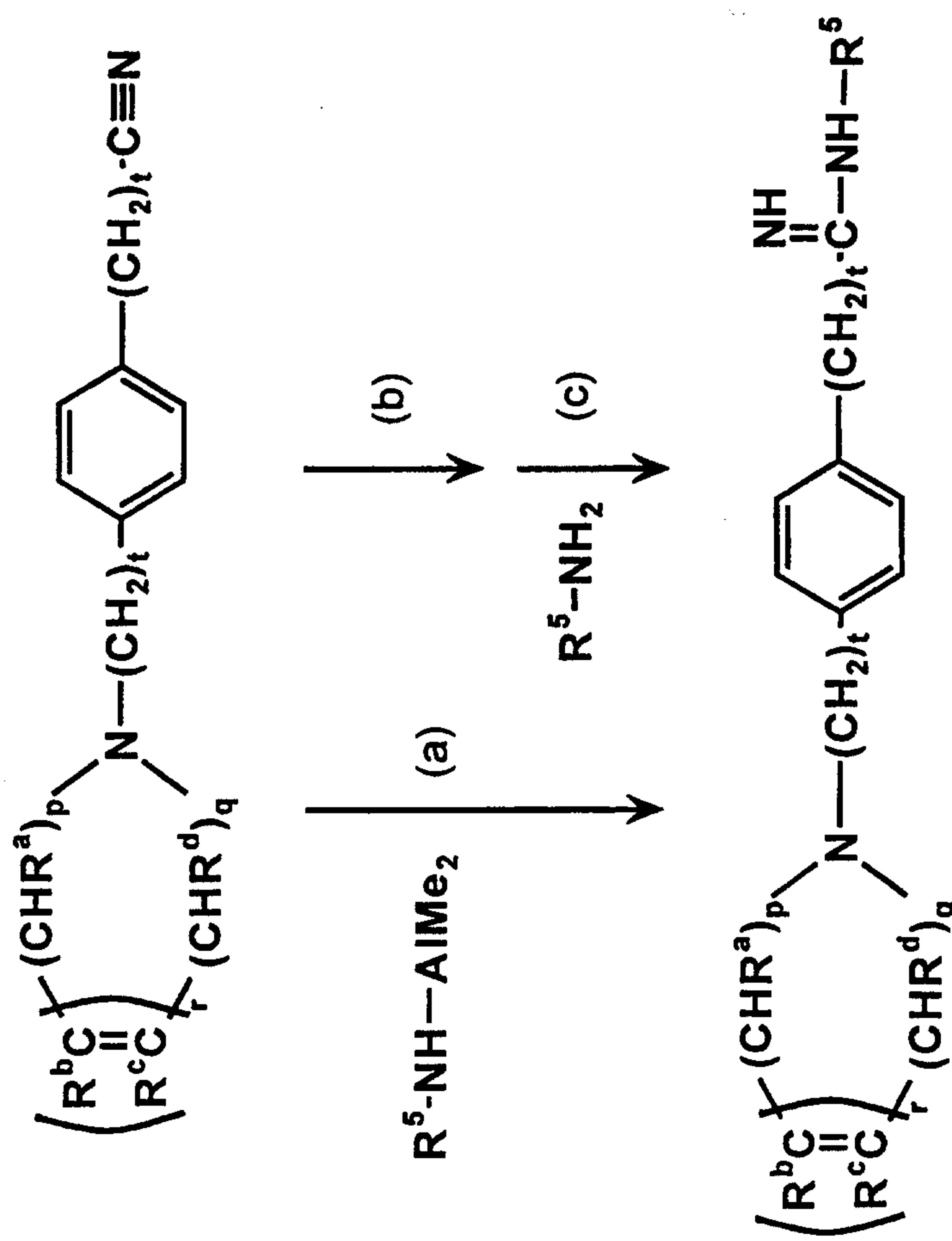
SCHEME 11:
