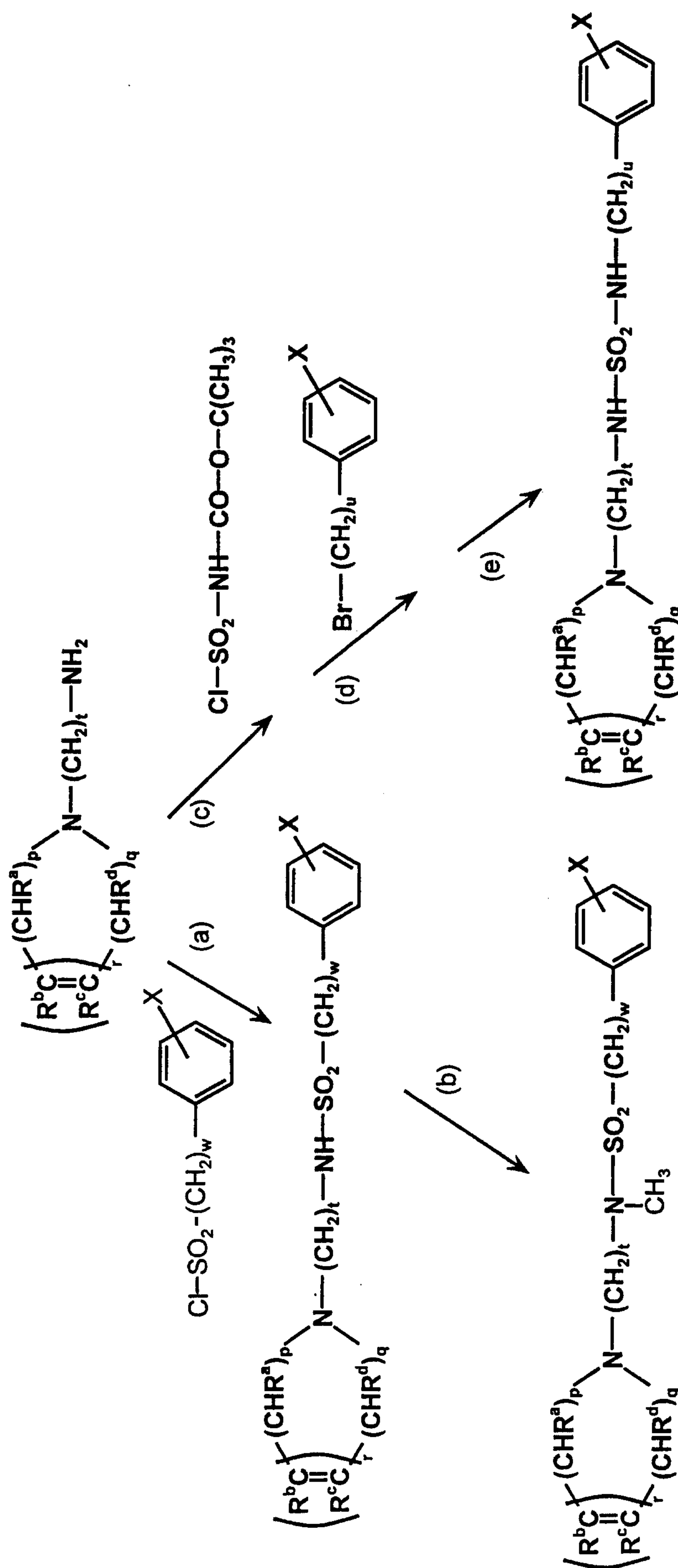
SCHEME 12
