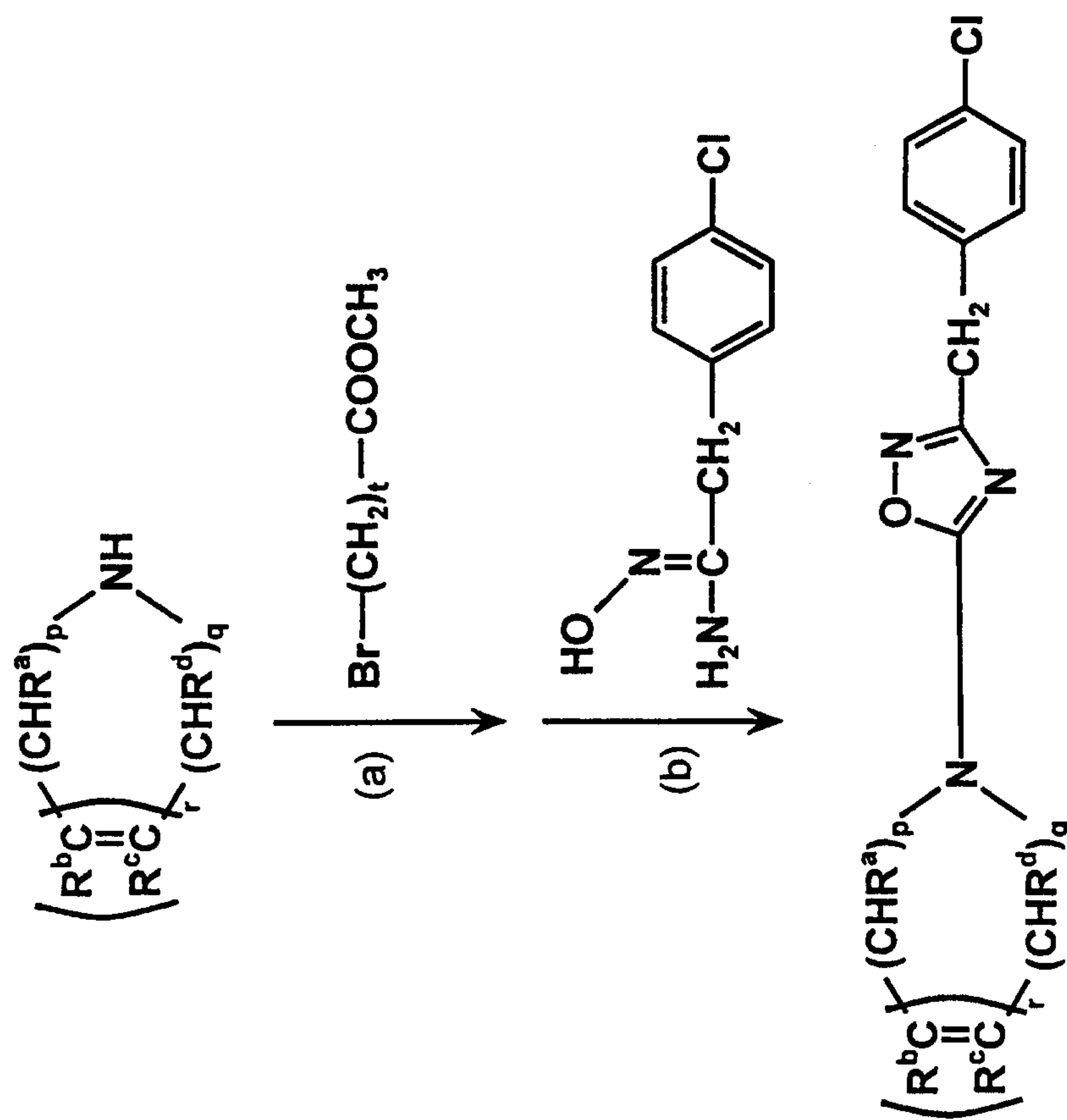
SCHEME 10:
