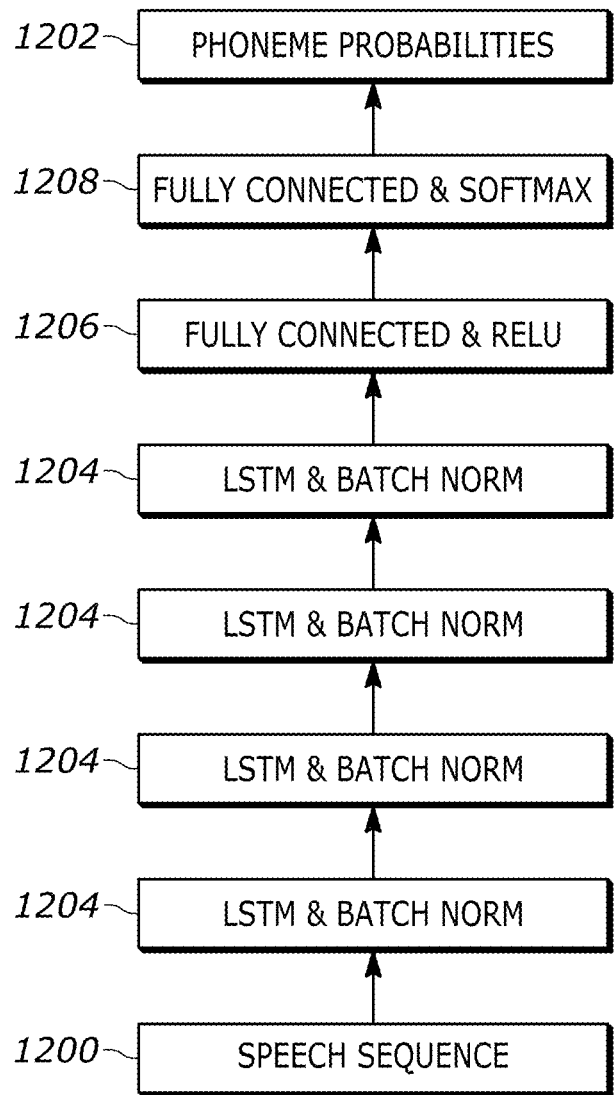
PHONEME RECOGNIZER ARCHITECTURE
