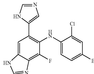
(4-Bromo-2-chloro-phenyl)-[4-fluoro-6-(3H-imidazol-4-yl)-1H-benzimidazol-5-yl]-amine (10aa)
