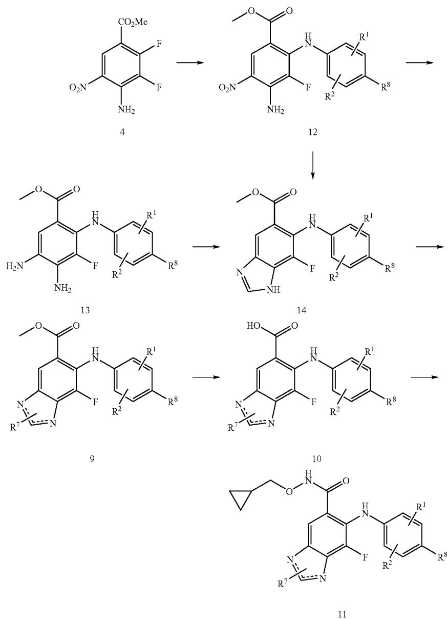
Scheme 2
