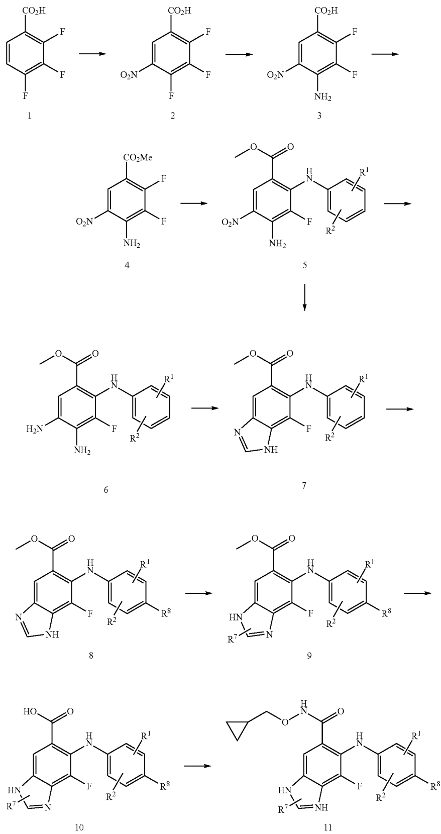
Scheme 1
