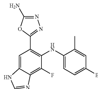
[6-(5-Amino-[1,3,4]oxadiazol-2-yl)-4-fluoro-1H-benzimidazol-5-yl]-(4-bromo-2-methyl-phenyl)-amine (24a)
