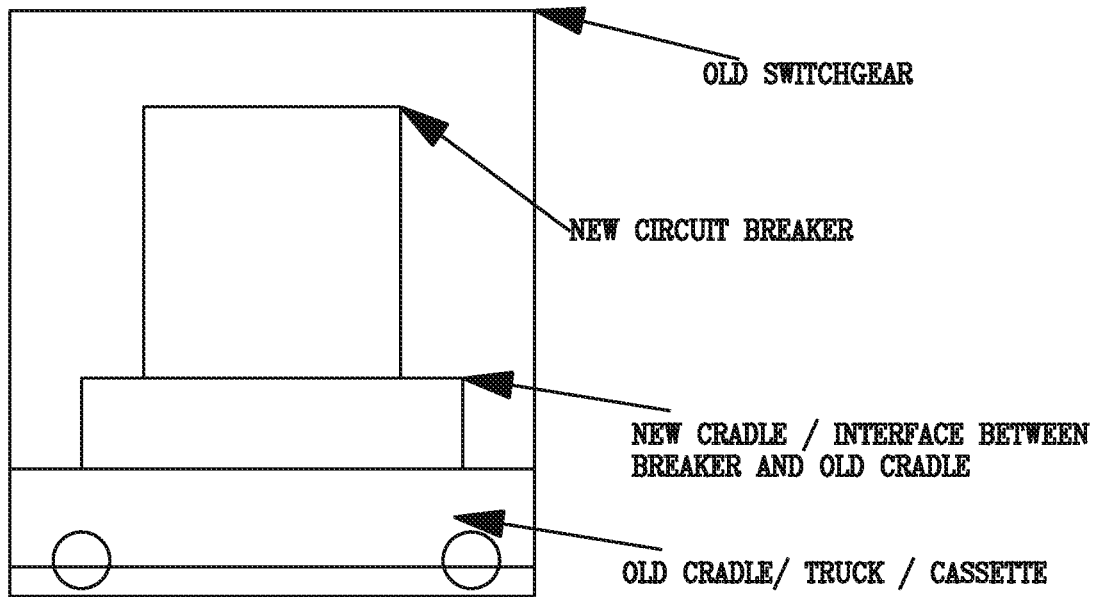
RETROFIT ARRANGEMENT - 2: ROLL IN
