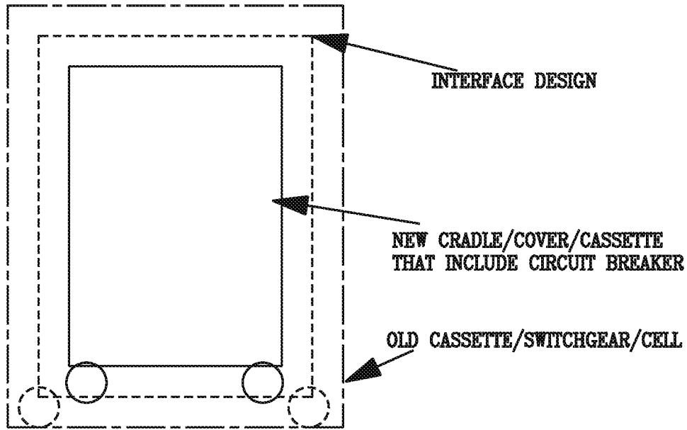
RETROFIT ARRANGEMENT - 1: CRADLE IN
