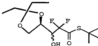
XVII/XVIII Anti/Syn = 85/15
