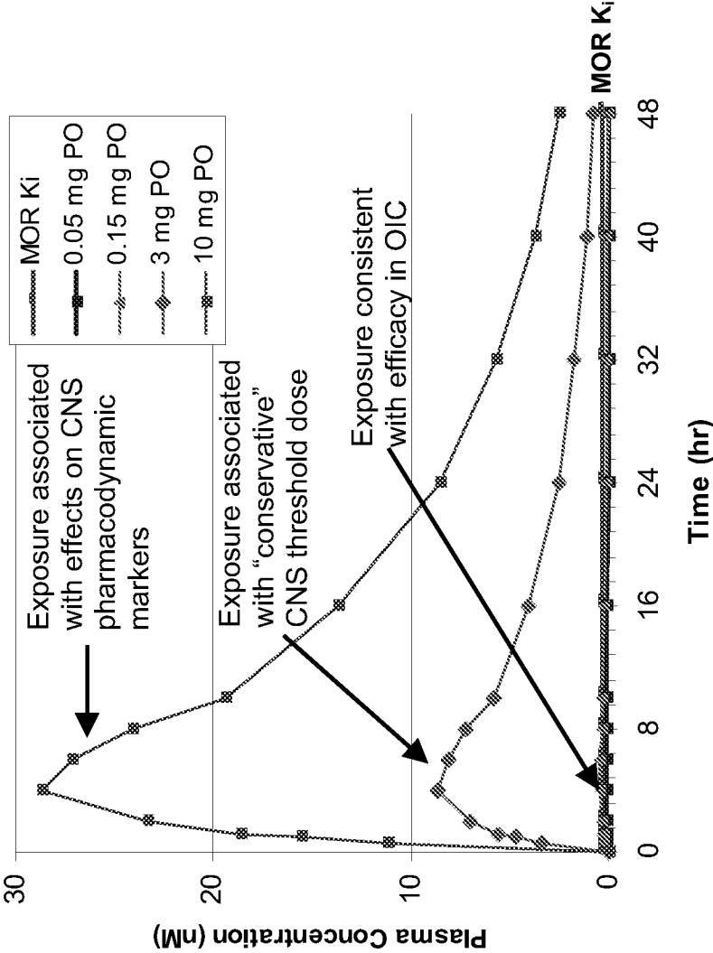
Figure 4 Measured (3 and 10 mg) and Modelled (0.05 and 0.15 mg) Free Plasma Concentration vs. Time Profile of Compound I in Humans (PO Doses)
