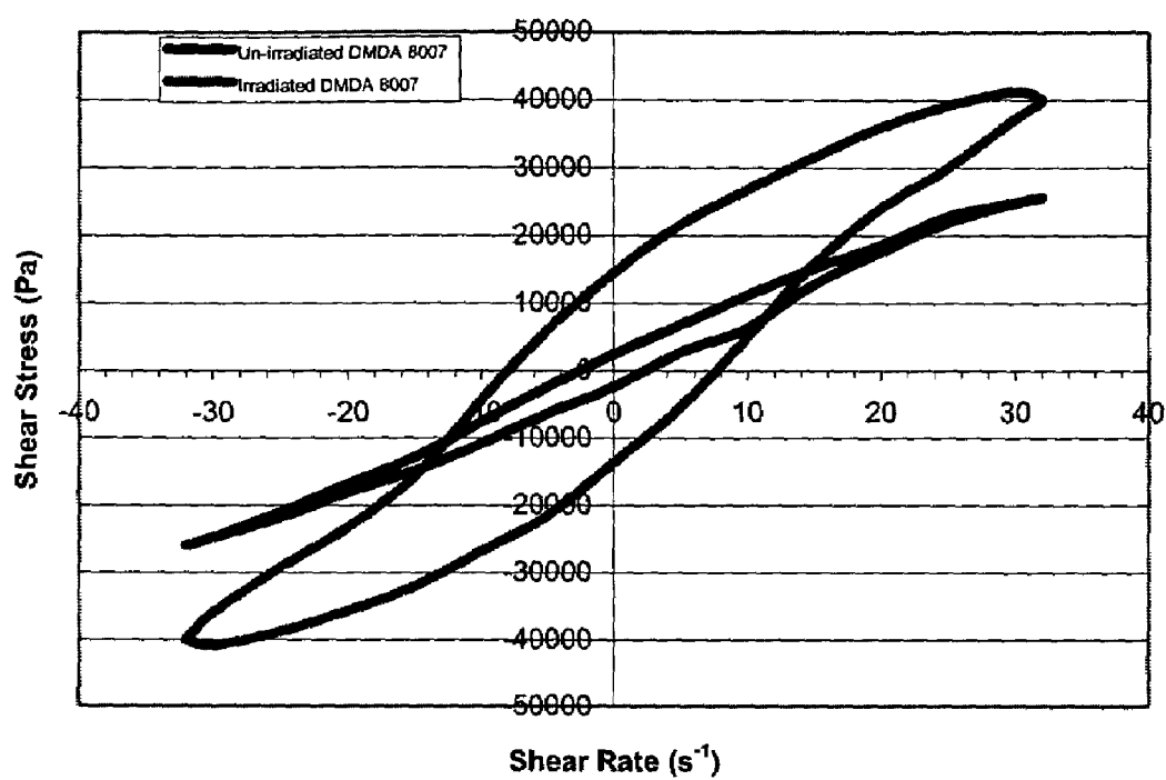
LAOS Curves For Irradiated And Un-Irradiated DMDA 8007
