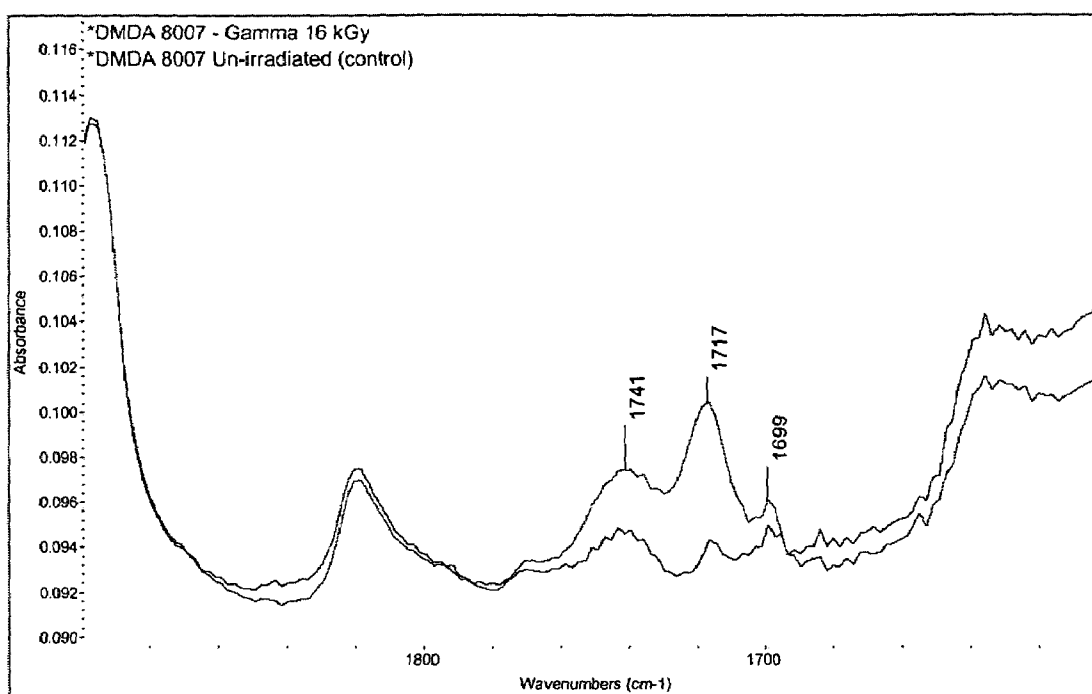
FTIR Spectra For Irradiated And Un-Irradiated DMDA 8007
