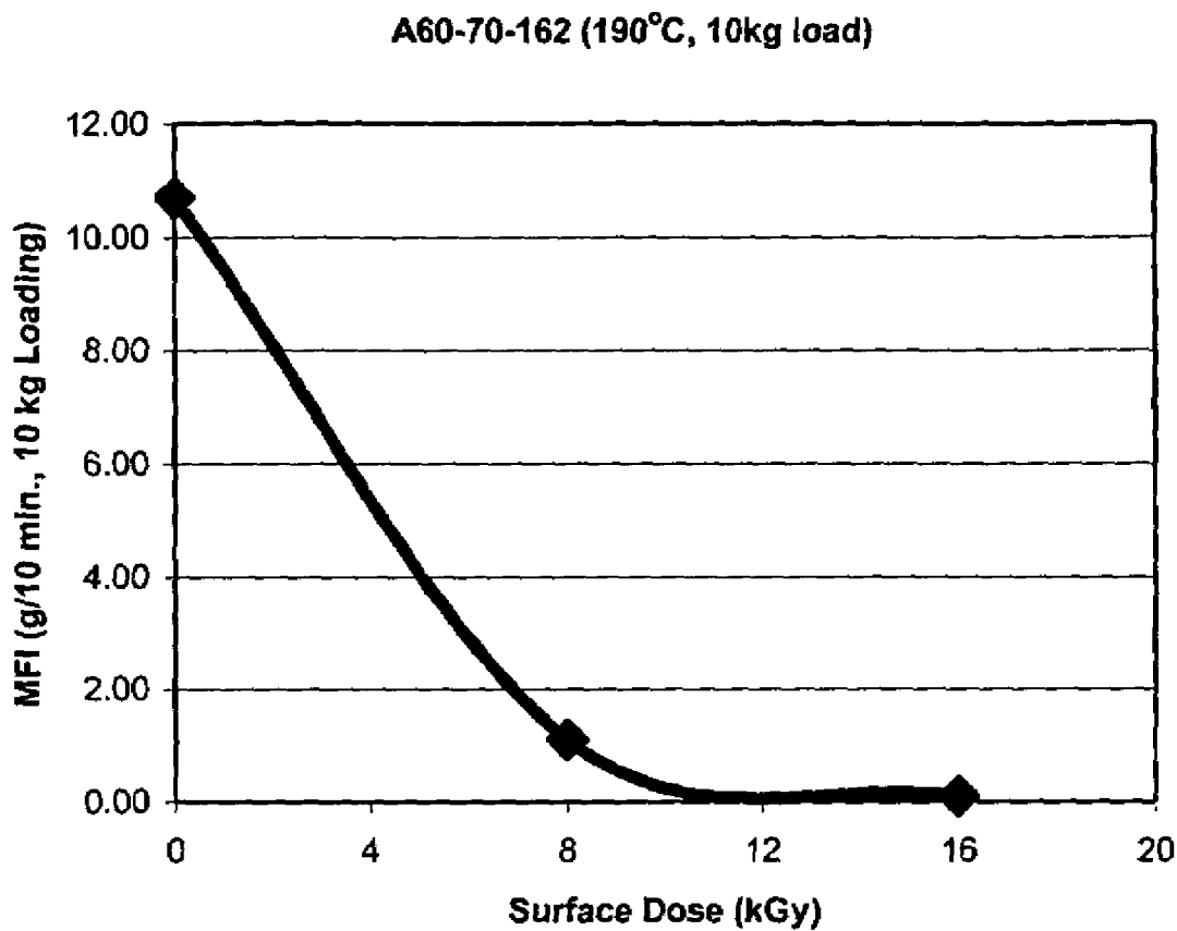
Melt flow Index of A60-70-162 Versus Surface Dose
