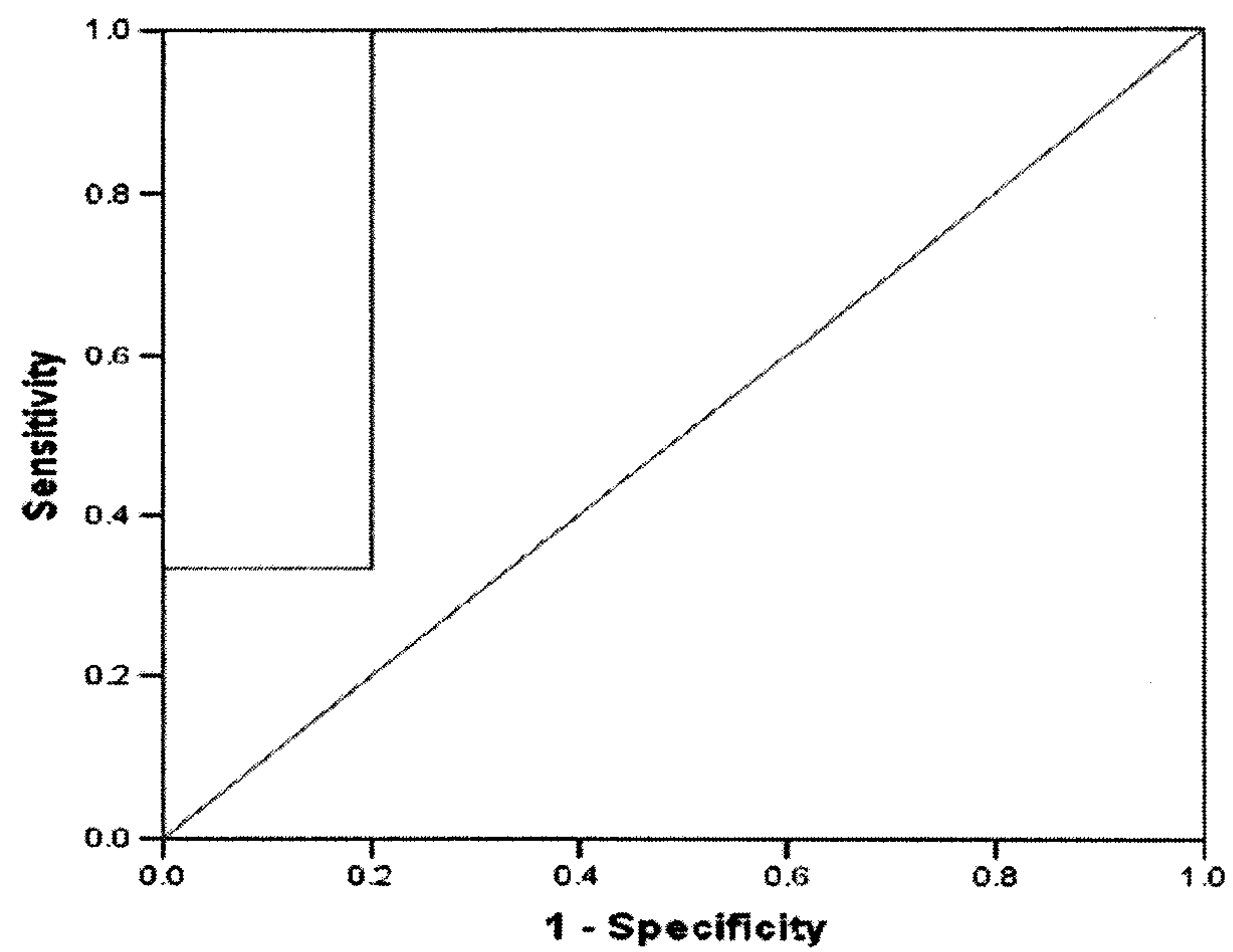
ROC Curve
