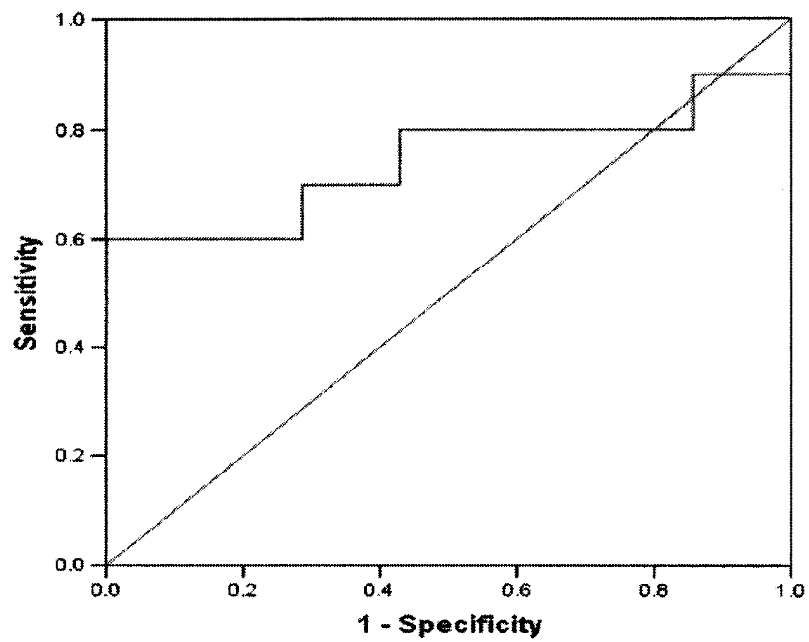
ROC Curve
