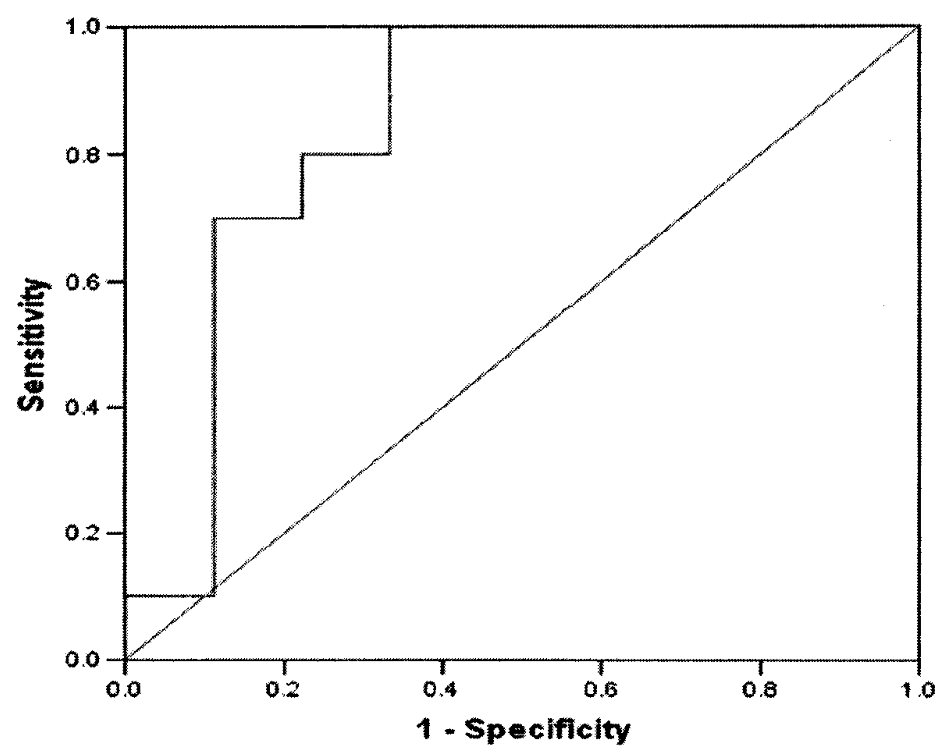
ROC Curve
