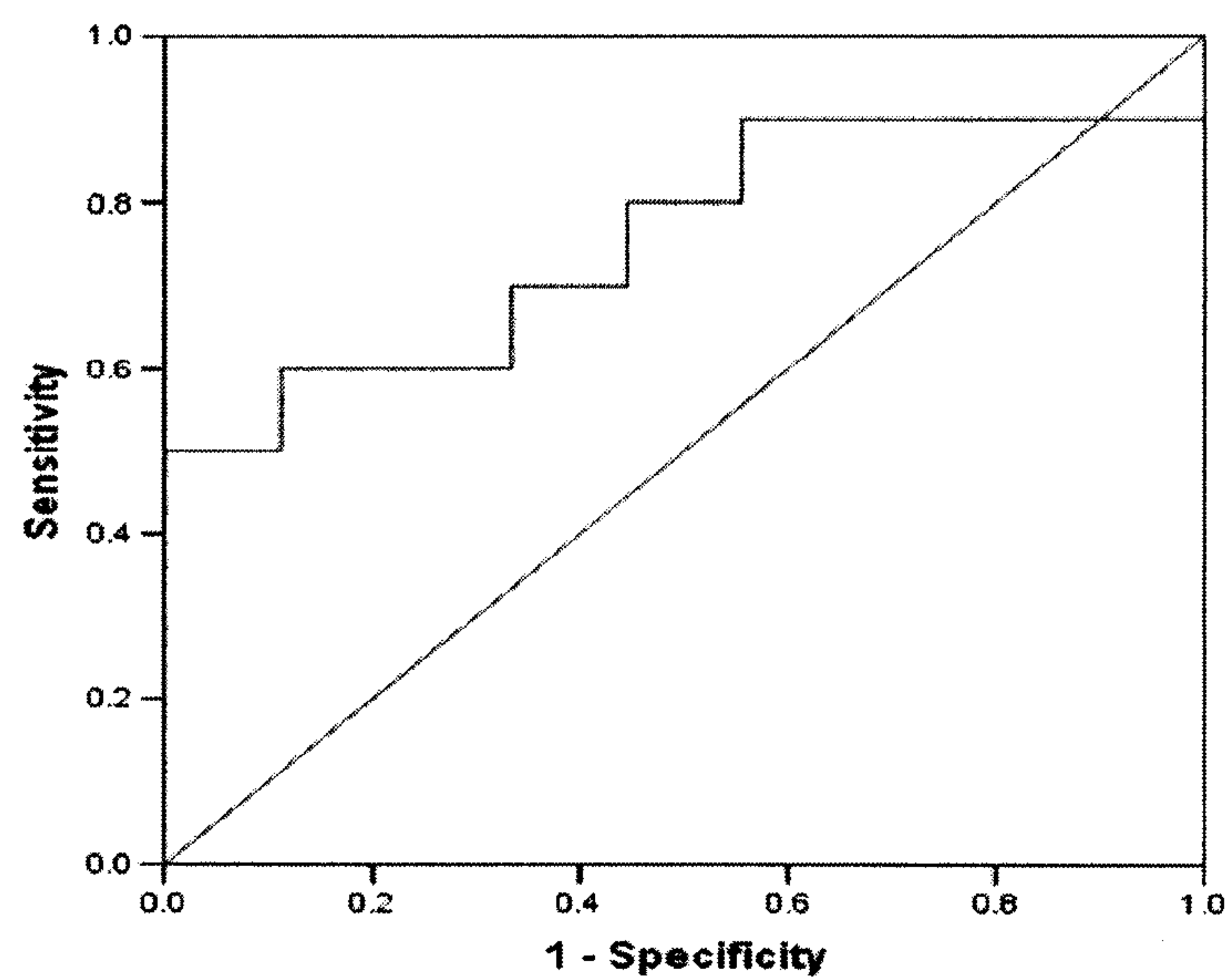
ROC Curve
