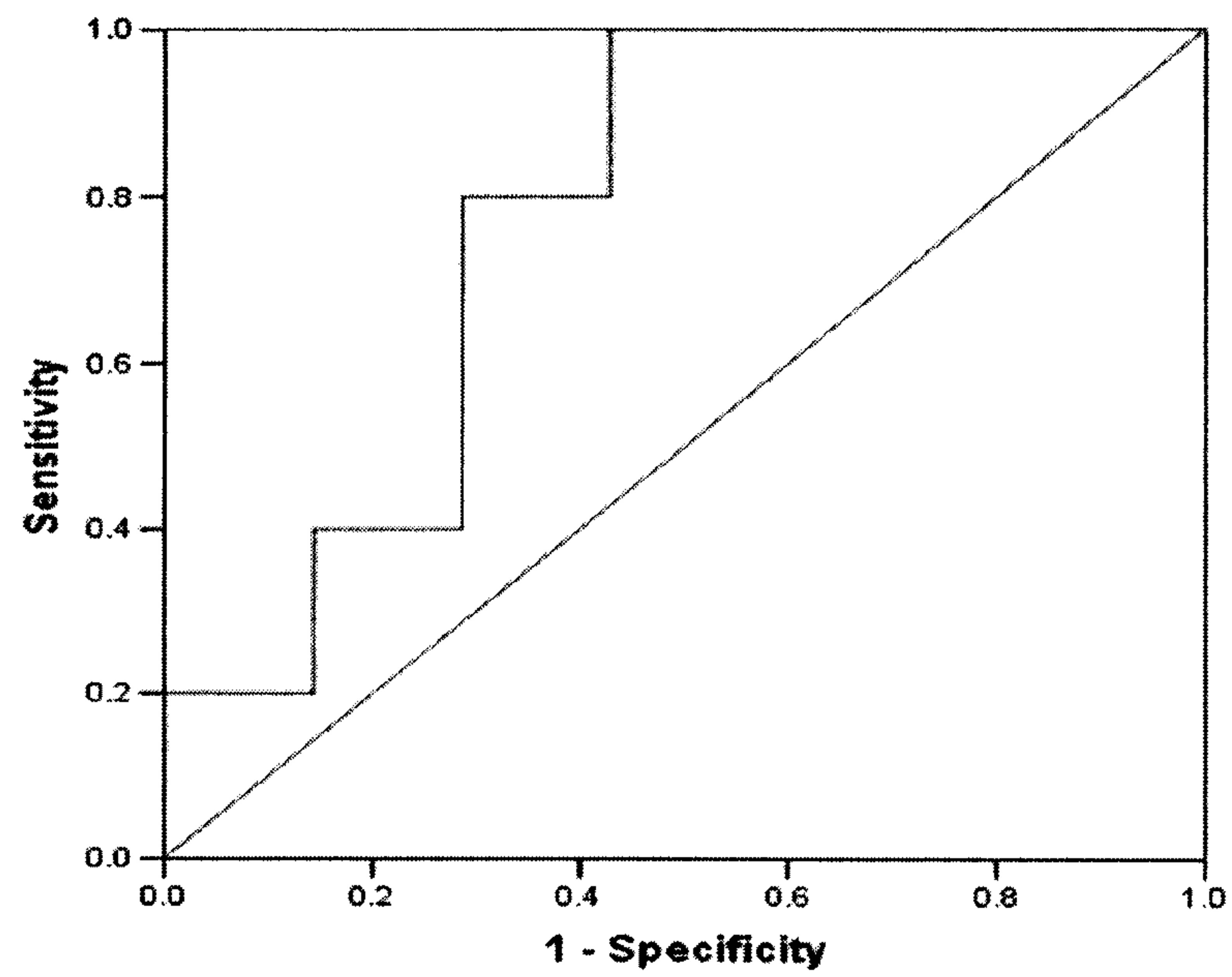
ROC Curve
