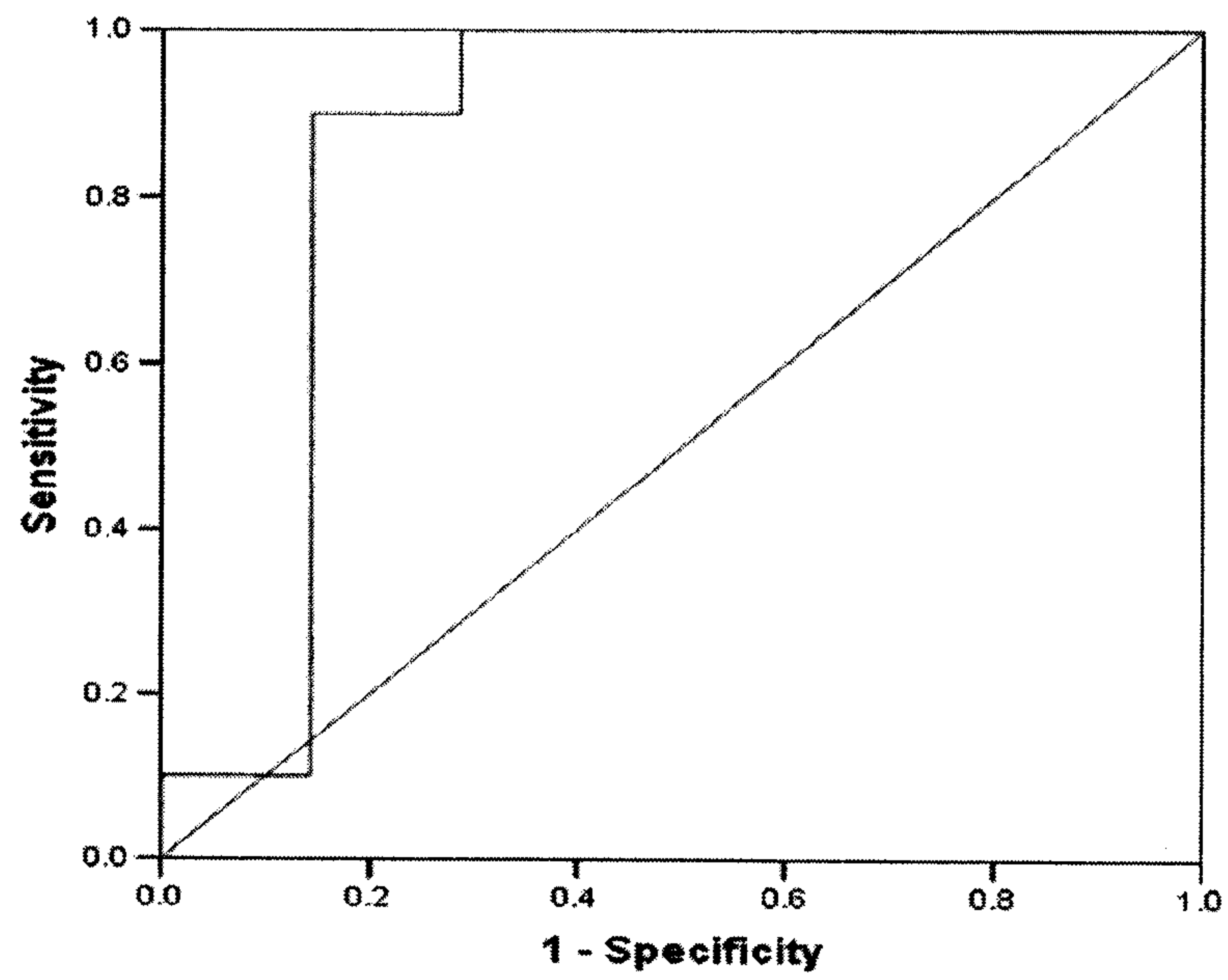
ROC Curve
