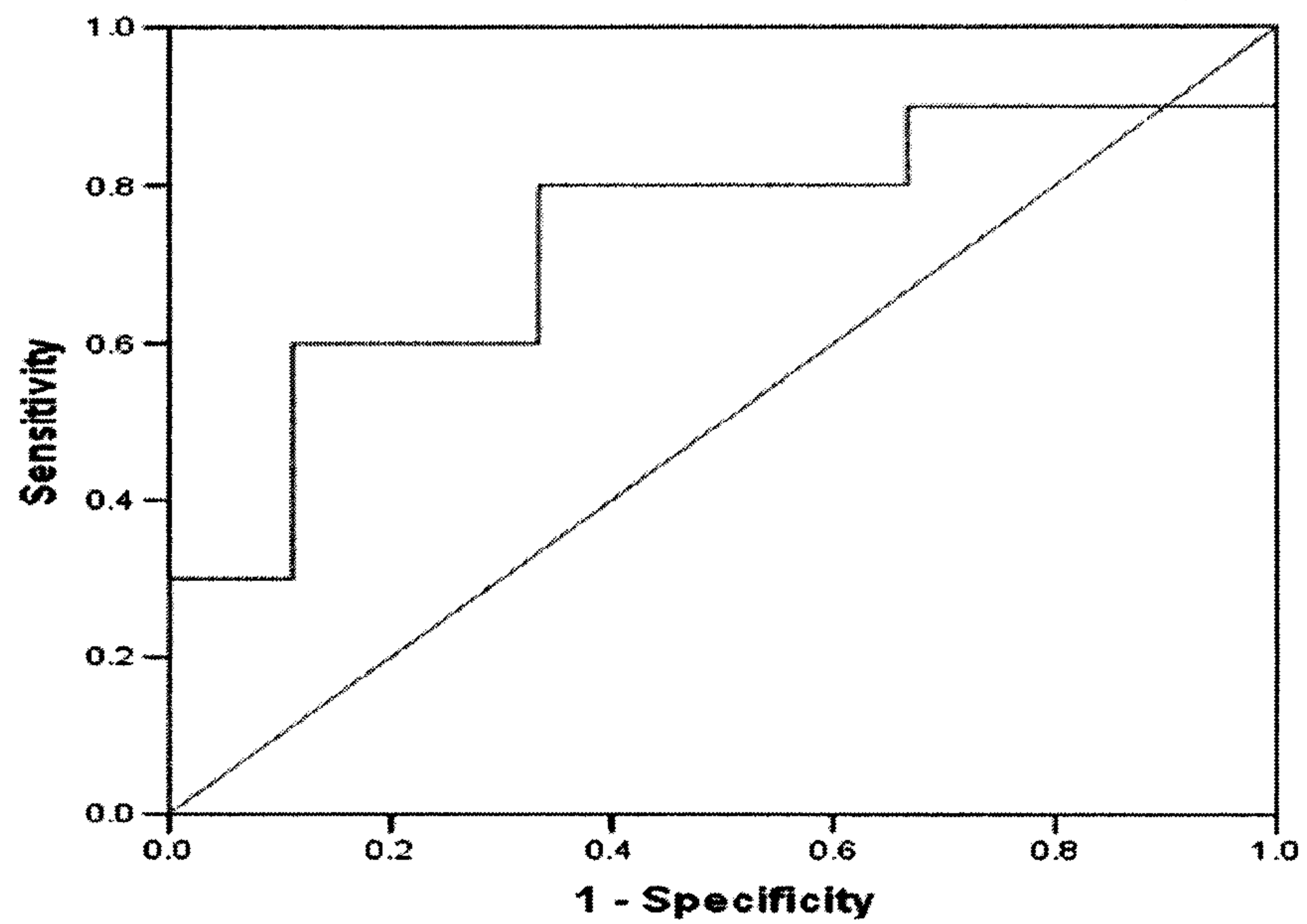
ROC Curve
