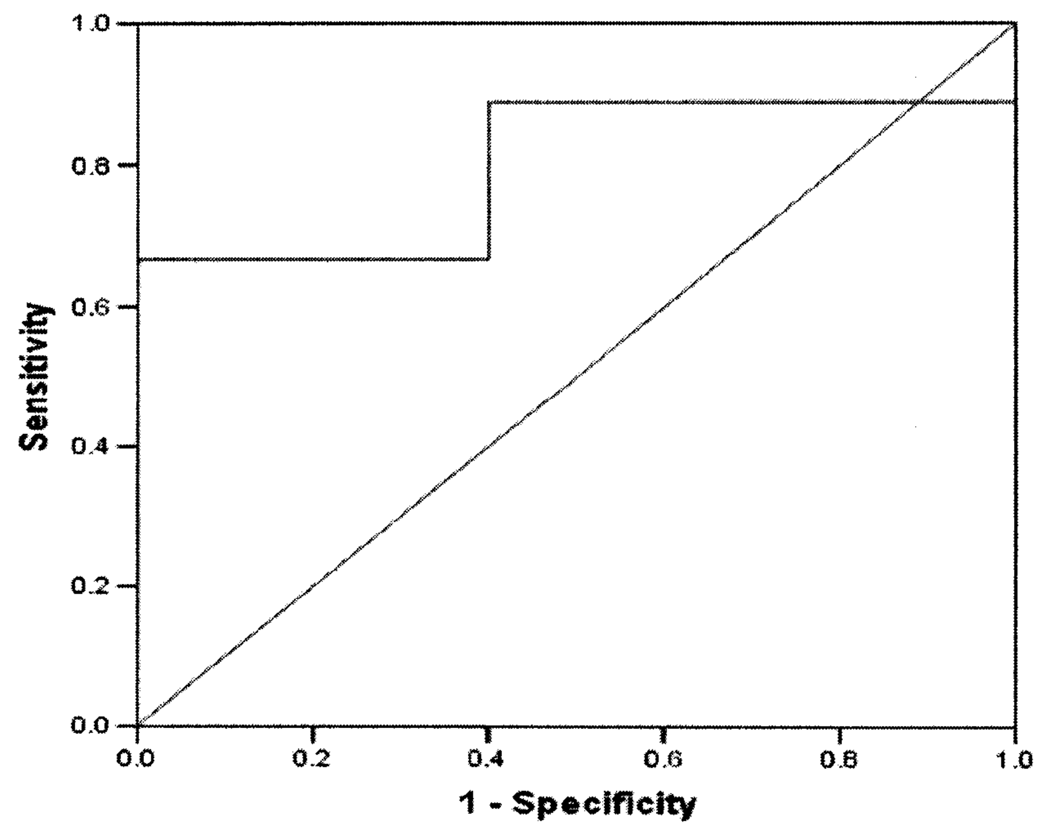
ROC Curve
